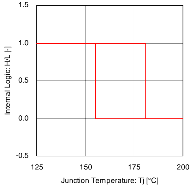
Fig.22 Thermal shutdown
