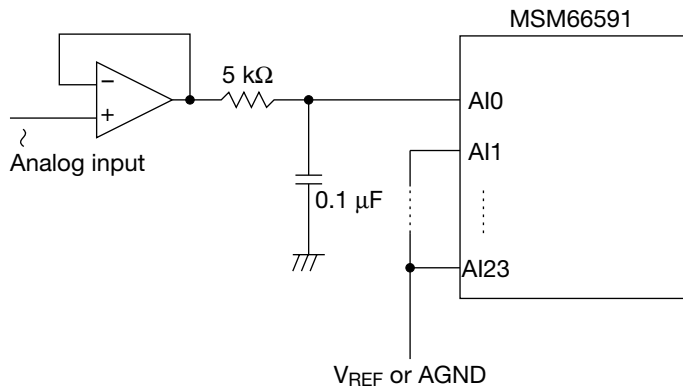
Figure 25-2 Crosstalk Measurement Circuit (MSM66591)
