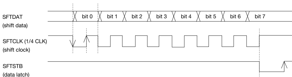
Figure 22-4 Output Mode Timing (8-Bit Mode Example)
