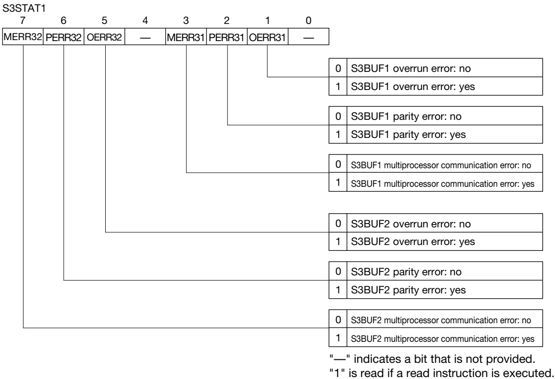
Figure 15-21 Configuration of S3STAT1
