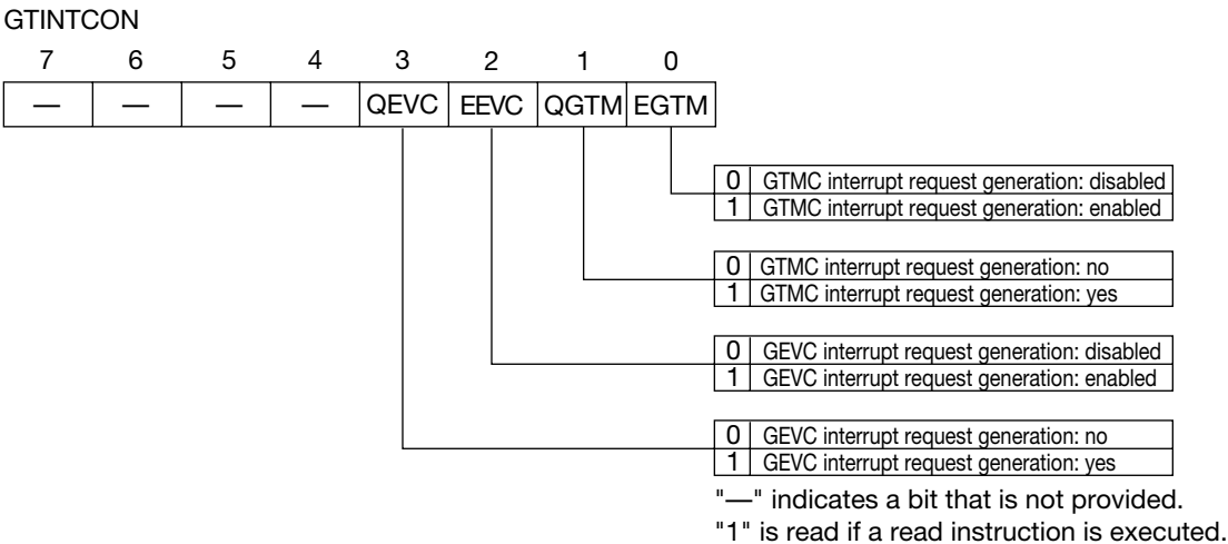
Figure 12-3 GTINTCON Configuration
