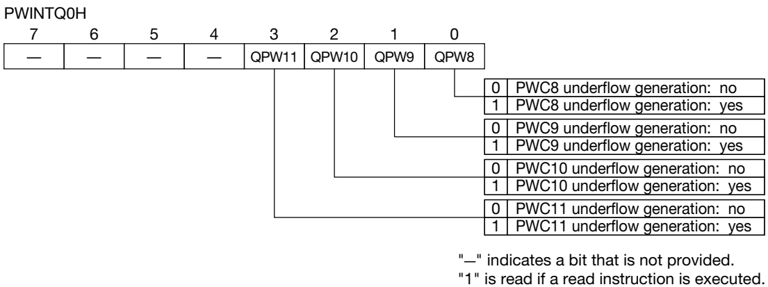
Figure 13-11 Configuration of PWINTQ0H
