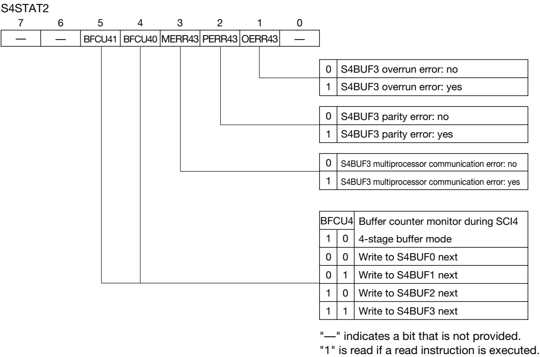
Figure 15-28 Configuration of S4STAT2
