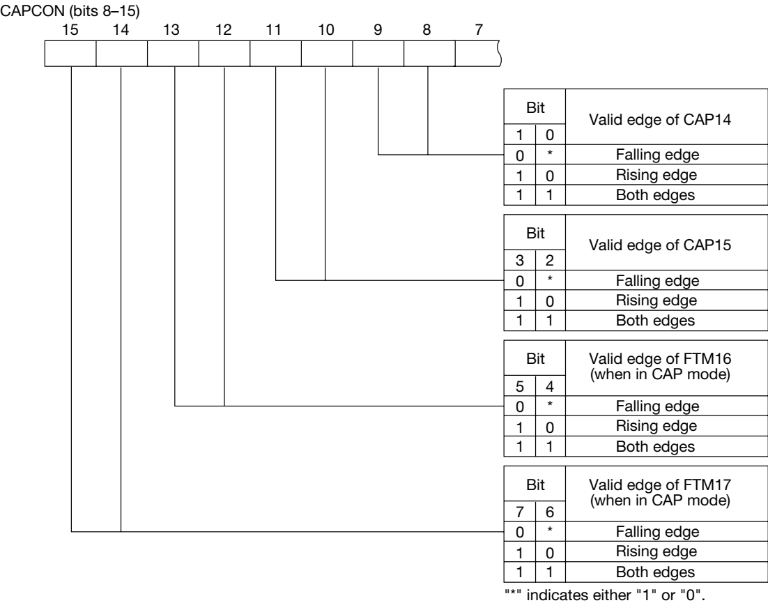
Figure 11-27 Configuration of Bits 8–15 of CAPCON
