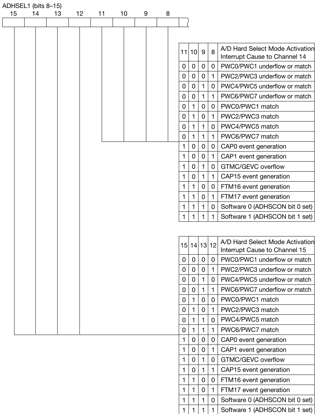
Figure 16-14 Configuration of ADHSEL1 (high-order bits)
