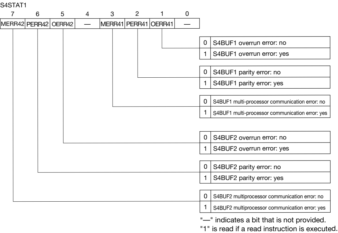
Figure 15-27 Configuration of S4STAT1
