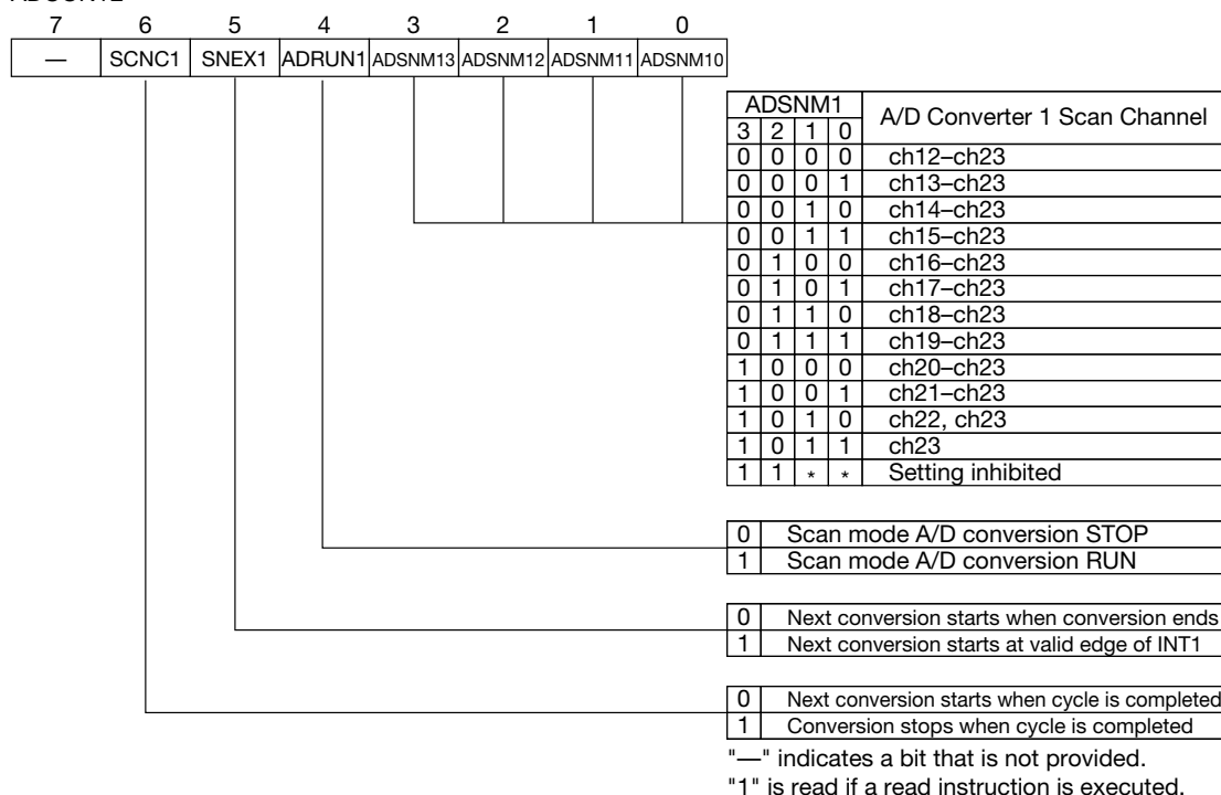
ADCON1L
