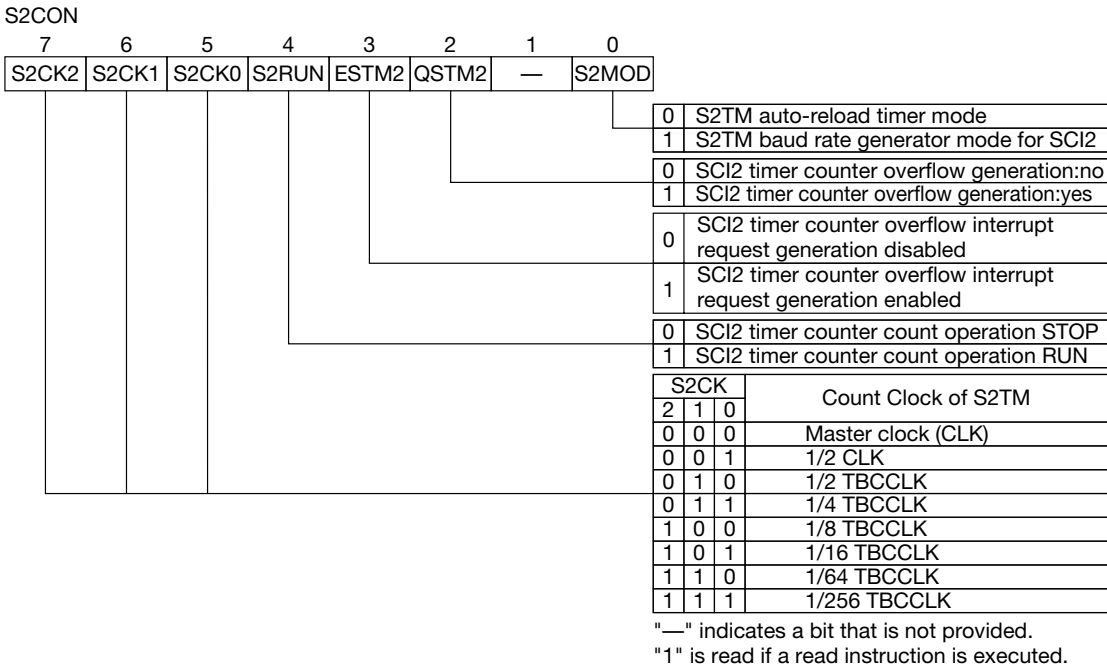
Figure 14-4 Configuration of S2CON
