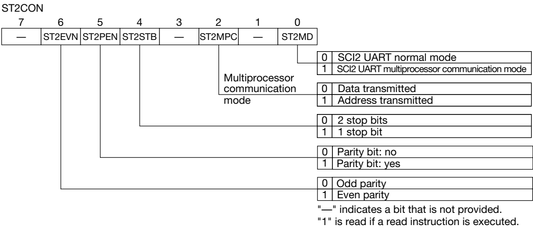
Figure 15-12 Configuration of ST2CON
