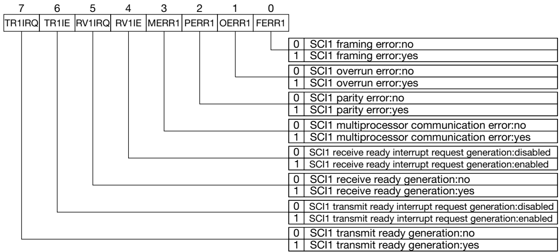
Figure 15-11 Configuration of S1STAT
