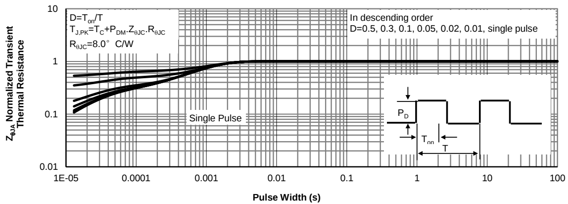
Figure 12: Normalized Maximum Transient Thermal Impedance (Note G)
