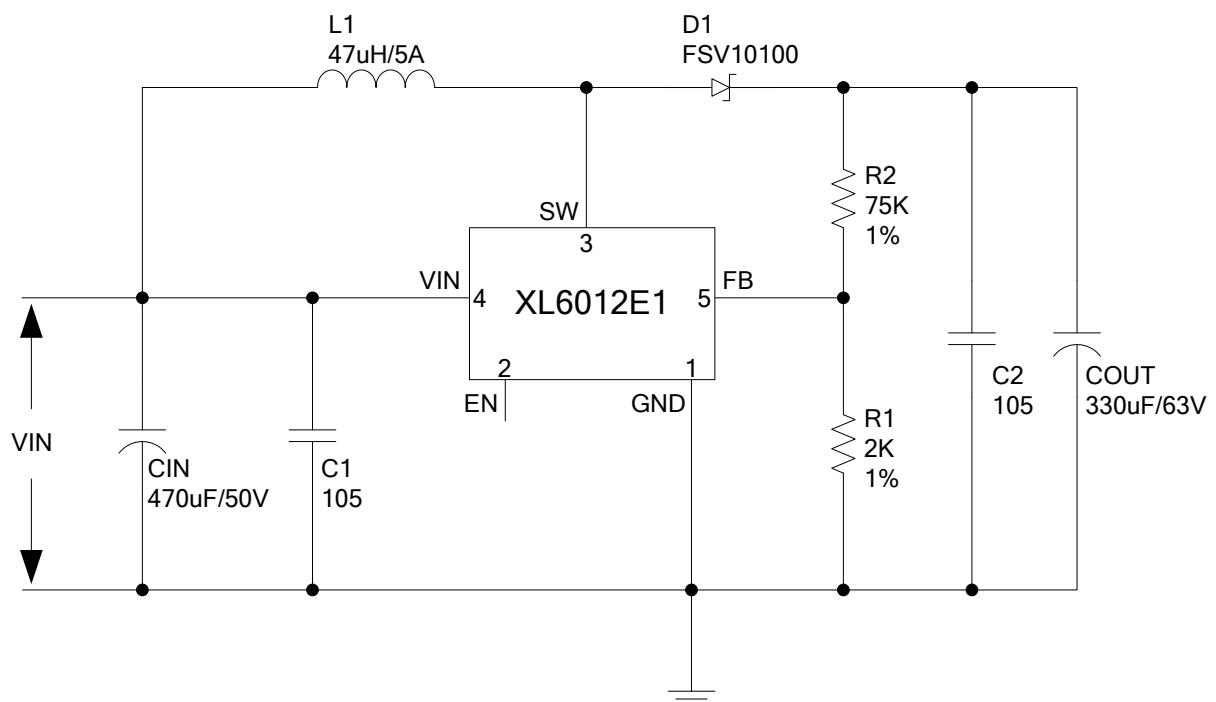
Figure20. XL6012 High Power Application Circuit (VIN=36V,VOUT=48V,IOUT=2.1A)
