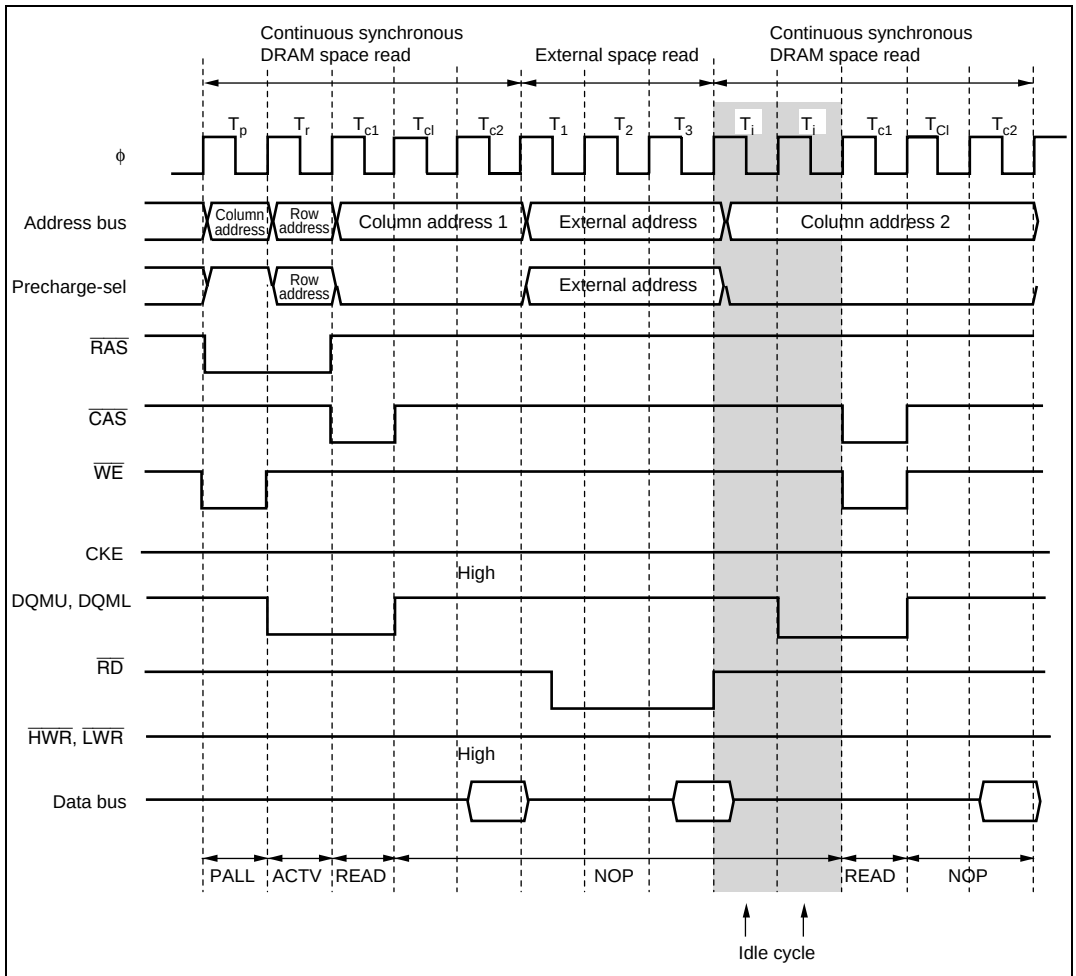
Figure 6.74 Example of Idle Cycle Operation in RAS Down Mode (Read in Different Area) (IDL = 1, CAS Latency = 2)
