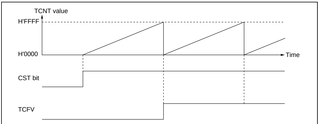
Figure 11.3 Free-Running Counter Operation
