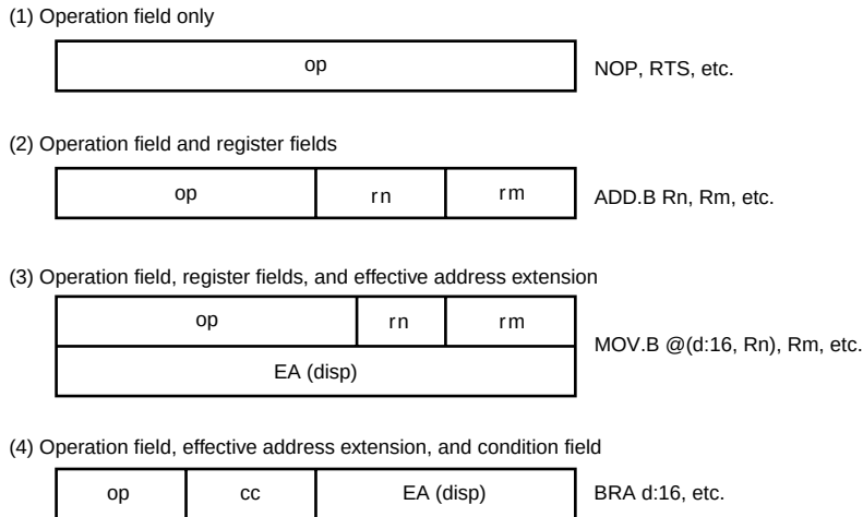
Figure 2.11 Instruction Formats (Examples)
