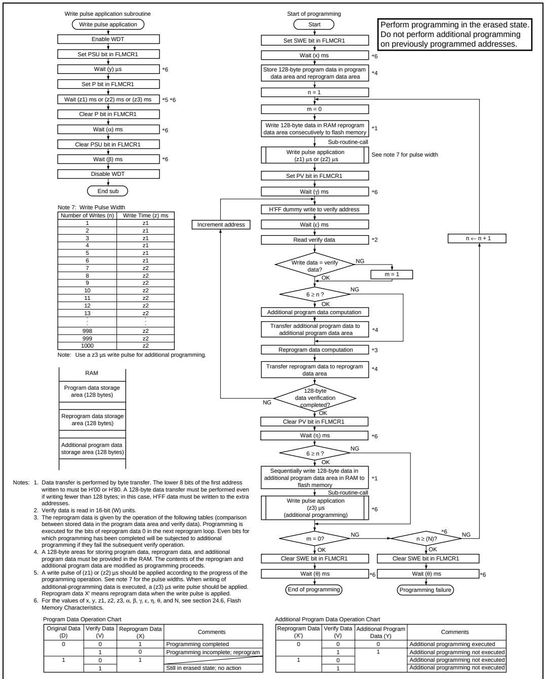
Figure 19.10 Program/Program-Verify Flowchart
