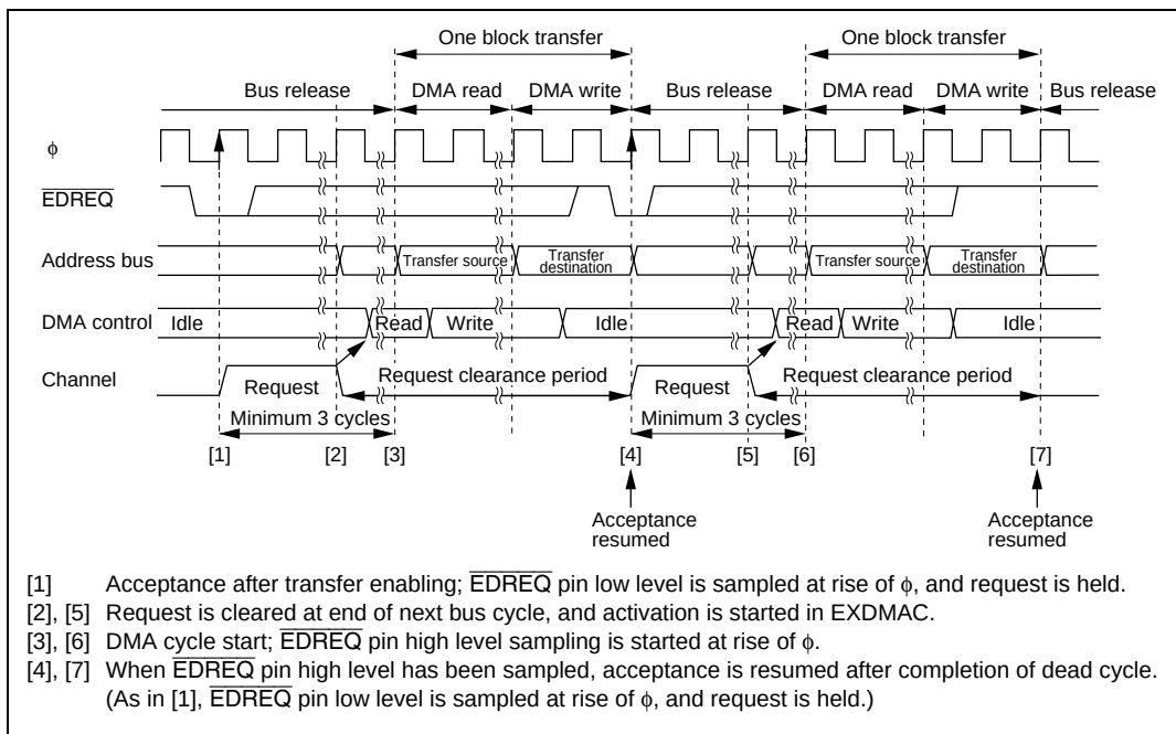
Figure 8.19 Example of Block Transfer Mode Transfer Activated by EDREQ Pin Falling Edge
