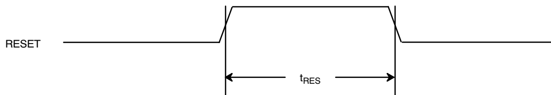
Figure 51. Reset Timing
