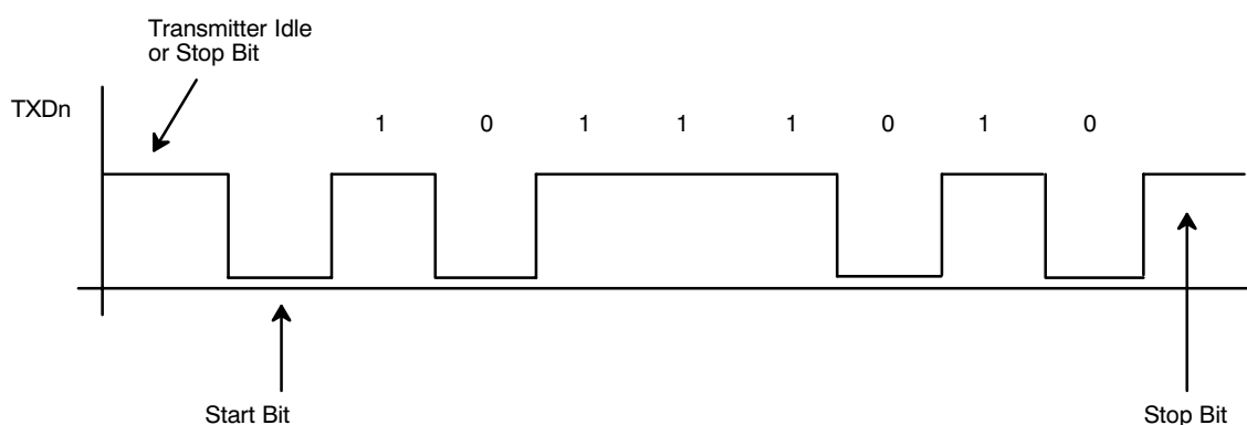
Figure 36. The Output Waveform of the Transmitter While Sending 5D 16 (8-N-1 Protocol).
