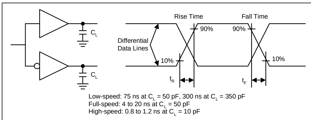
Figure 23-14. USB Jitter
