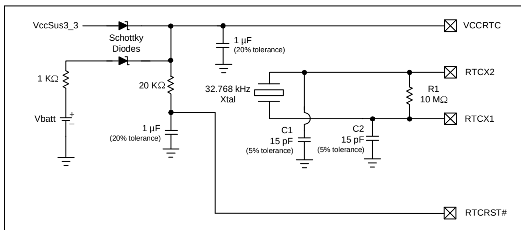
Figure 2-4. Example External RTC Circuit
