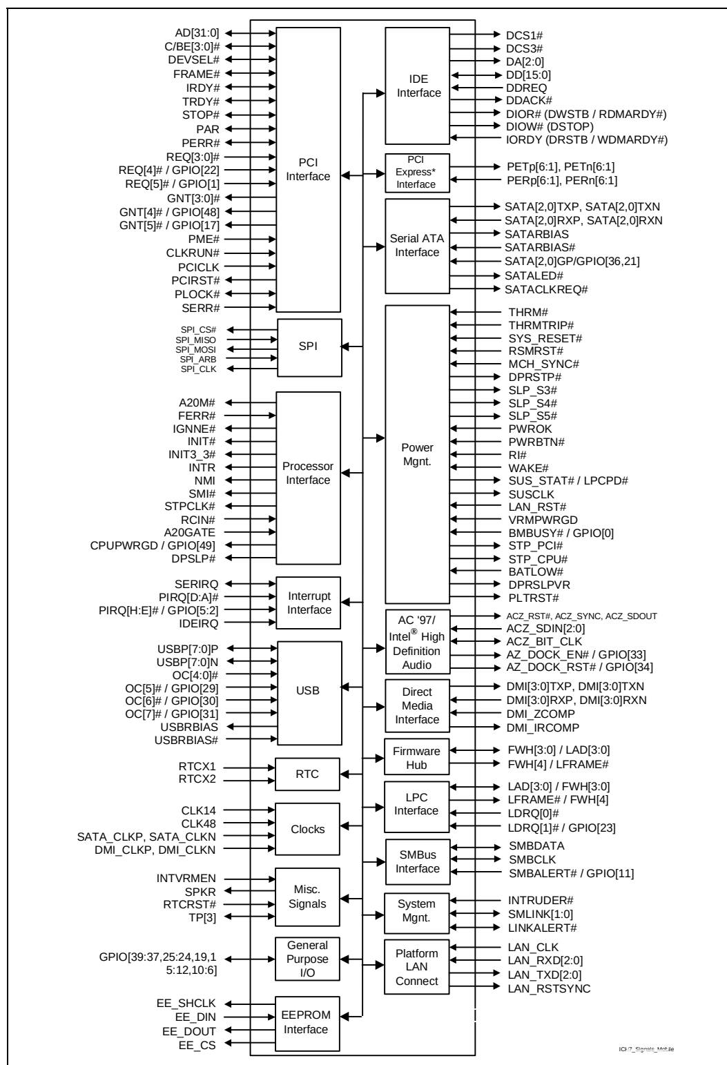
Figure 2-2. Interface Signals Block Diagram (Mobile Only)
