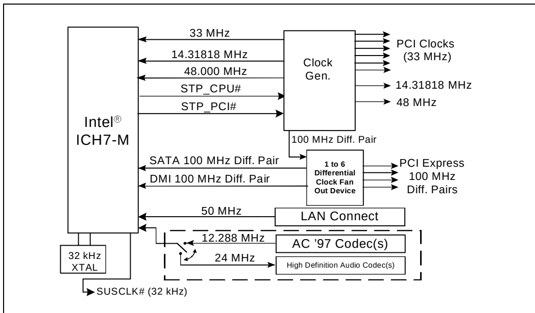
Figure 4-2. Mobile Only Conceptual Clock Diagram
