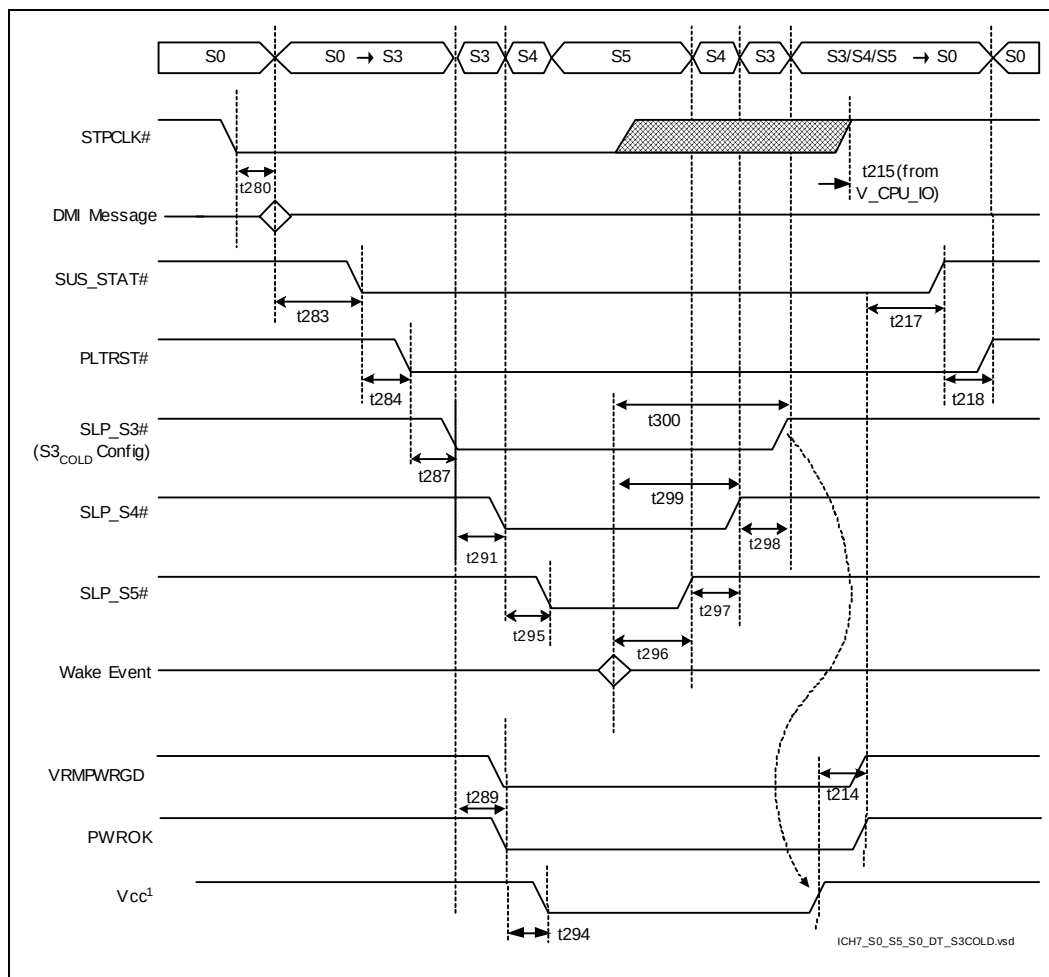
Figure 23-23. S0 to S5 to S0 Timings, S3 COLD (Desktop Only)
