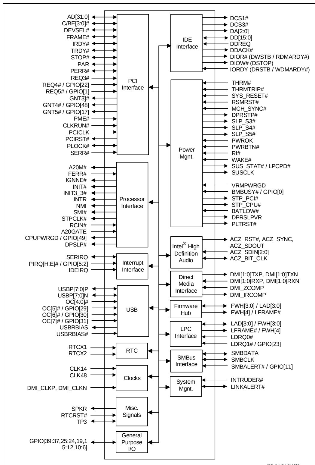
Figure 2-3. Interface Signals Block Diagram (Ultra Mobile Only)
