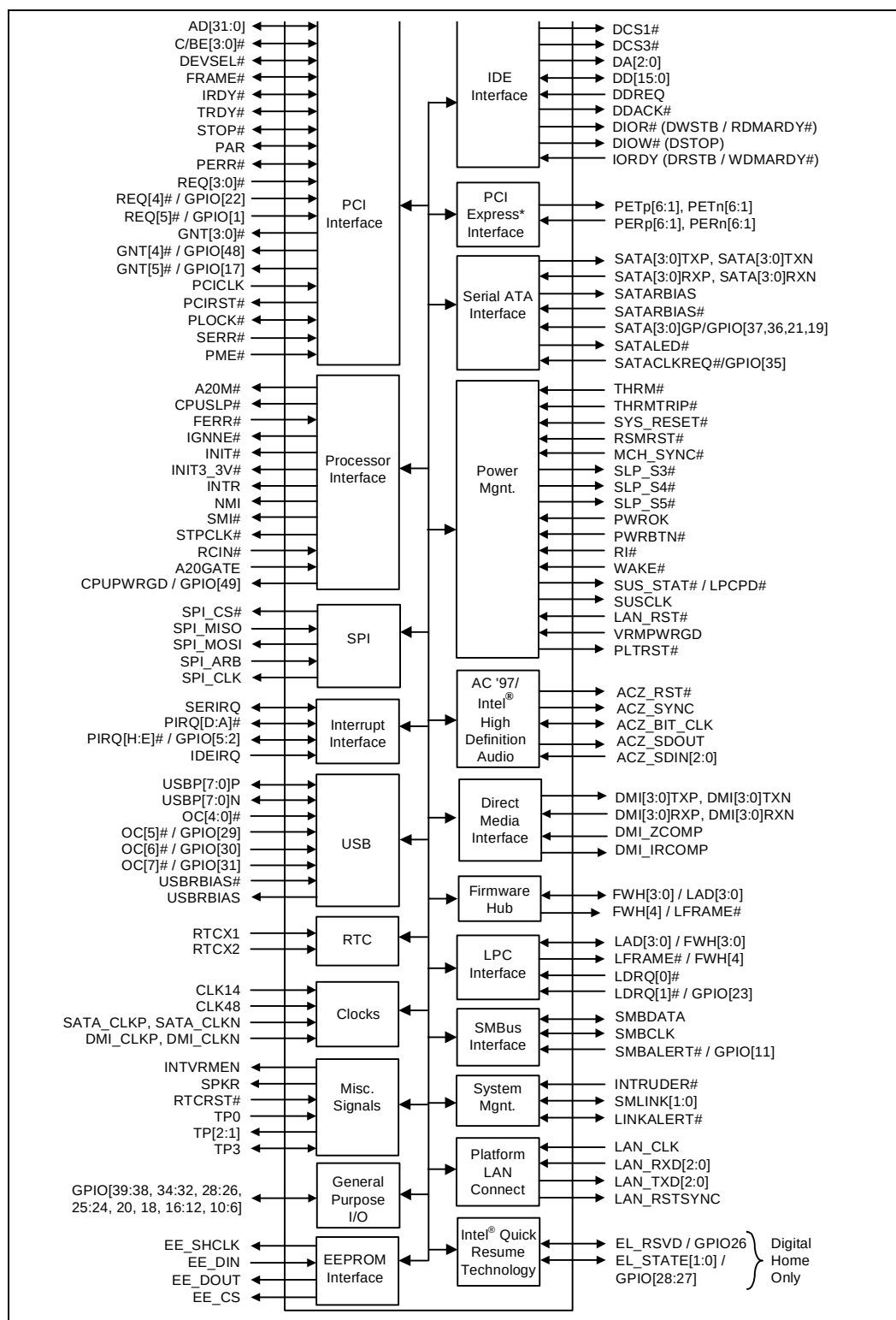
Figure 2-1. Interface Signals Block Diagram (Desktop Only)
