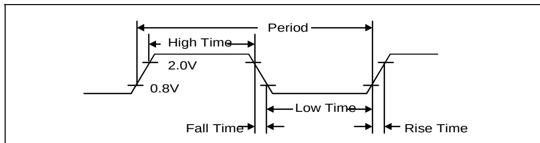
Figure 23-1. Clock Timing
