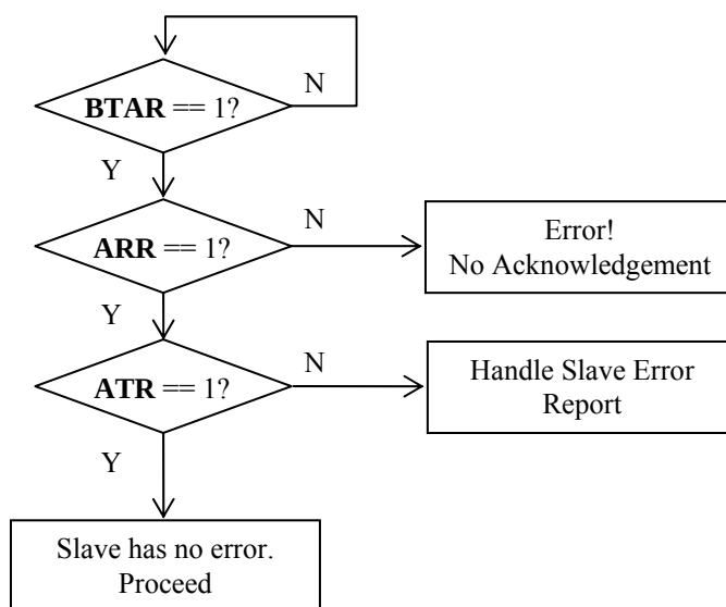
Figure 9-26: Acknowledgement Handling after Non-Read Command
