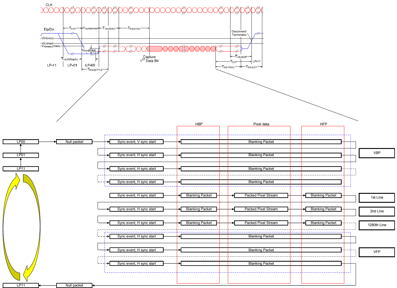
Figure 9-24: Non-Burst mode MIPI structure
