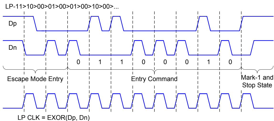
Figure 9-8: Trigger – Reset Command in Escape Mode
