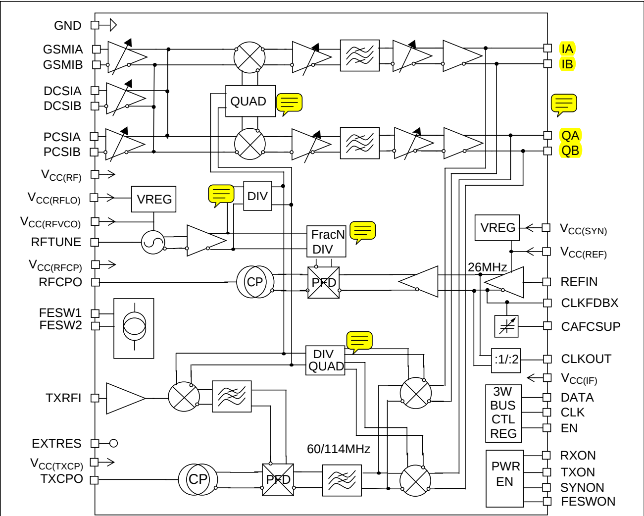
Fig.1 Block diagram.
