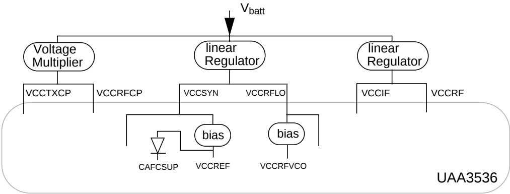
Fig.4 Power supply concept
