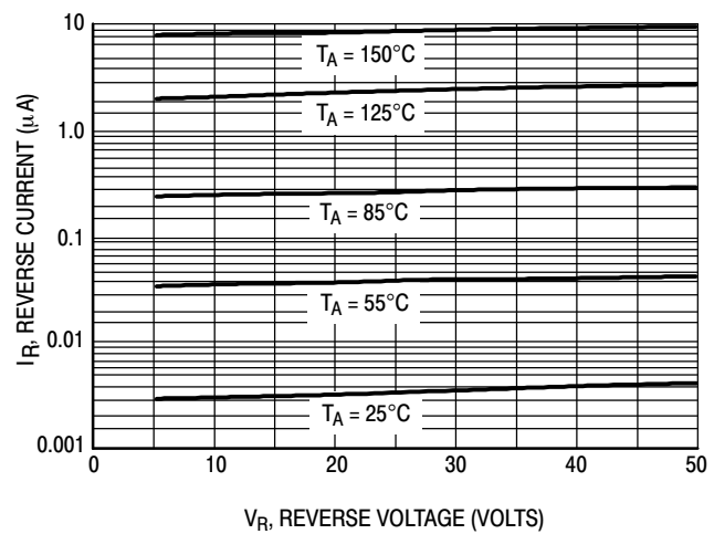
Figure 3. Leakage Current
