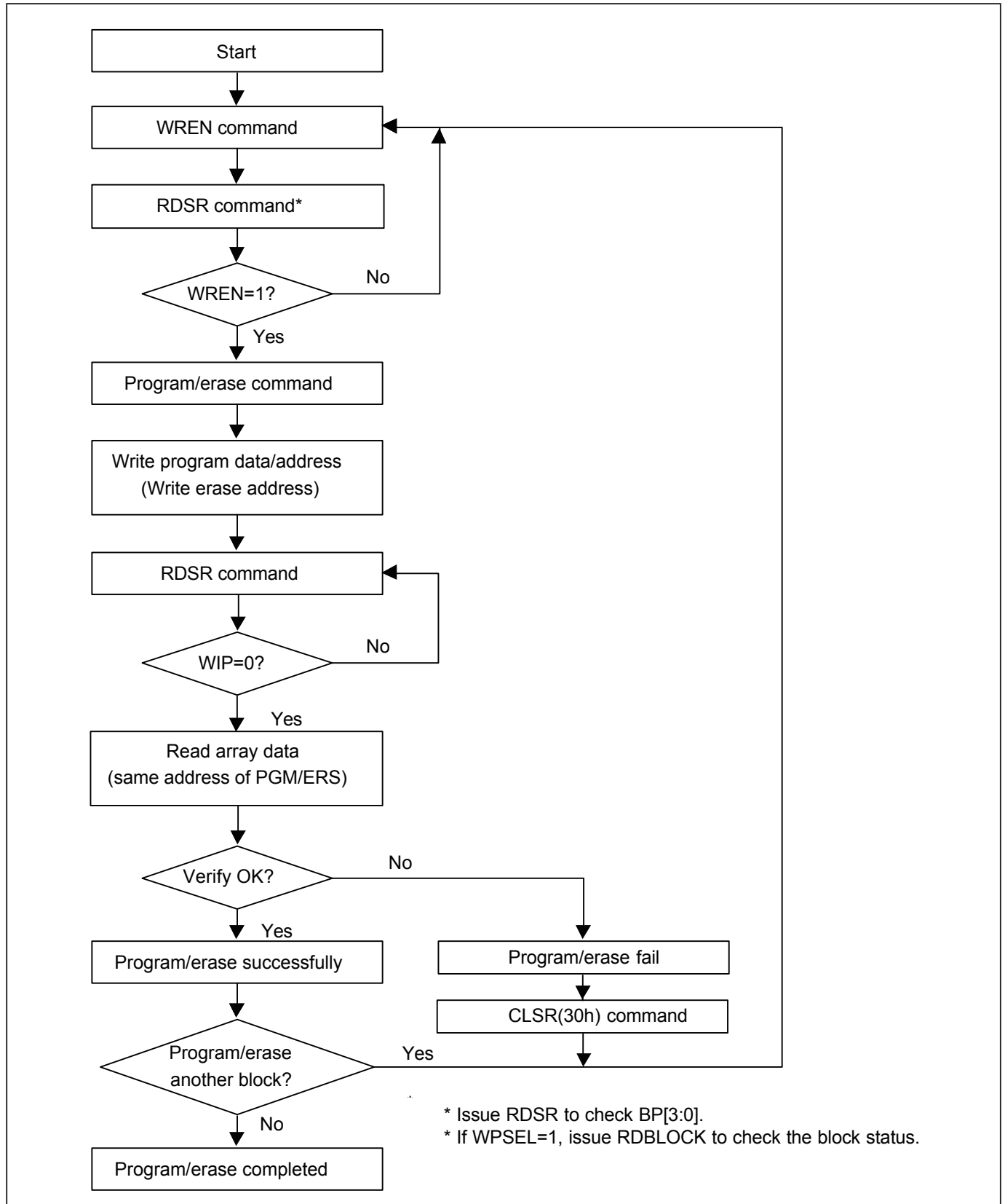
Figure 22. Program/Erase Flow(1) with read array data
