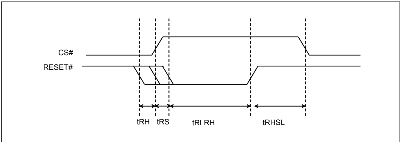
Figure 50. RESET Timing
