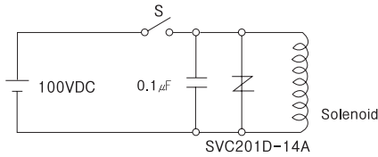
Contact protection
