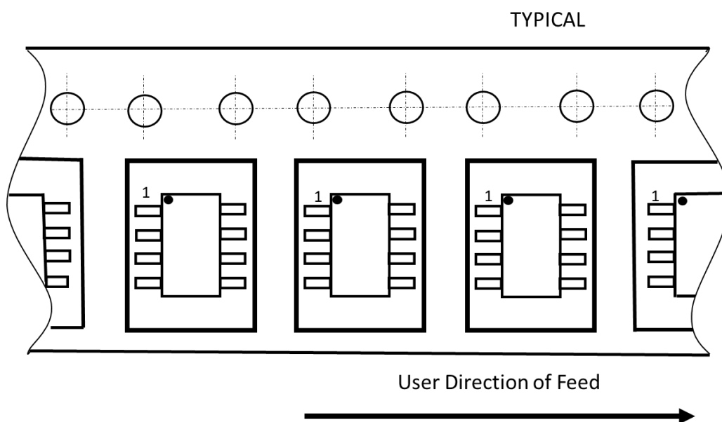
Figure 23. Tape orientation
