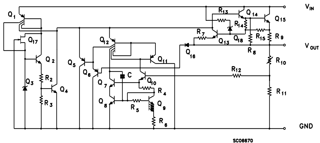
Figure 1. Schematic diagram
