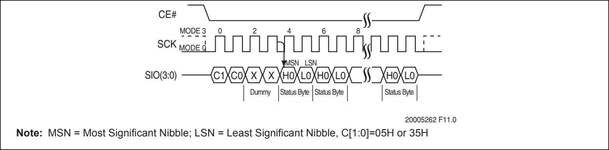
FIGURE 5-29: READ-STATUS-REGISTER AND READ-CONFIGURATION REGISTER SEQUENCE (SPI)
