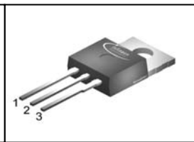
PG-TO220-3-1
