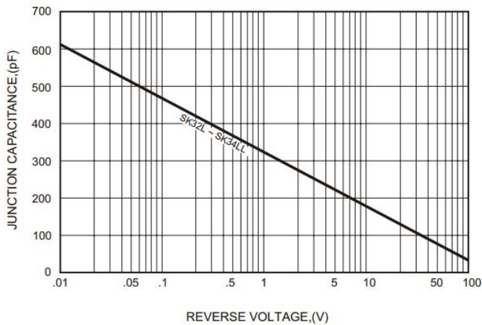
FIG.3-TYPICAL JUNCTION CAPACITANCE
