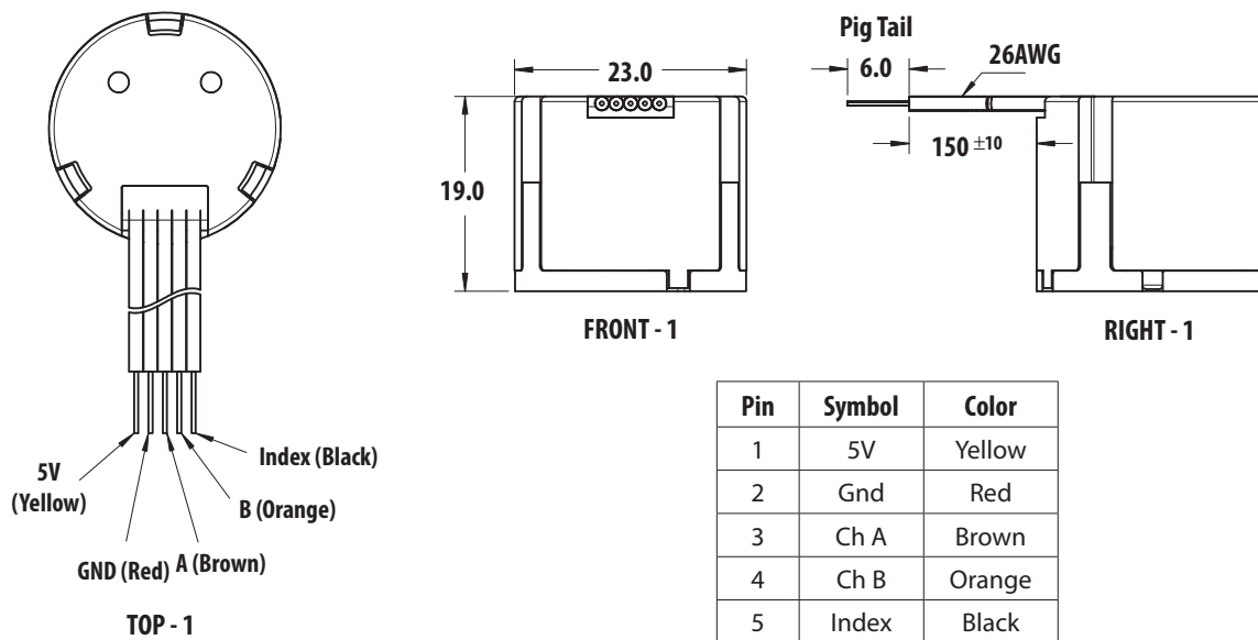
Figure 4. Electrical Connections
