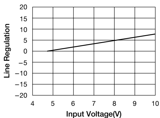
■ Line Regulation
