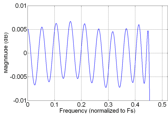
Inband ripple
