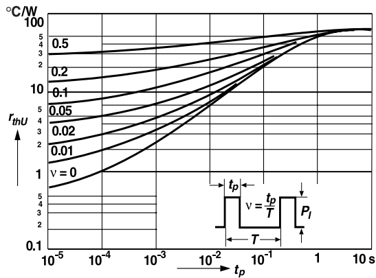
Figure 2. Pulse Thermal Resistance vs. Pulse Duration
