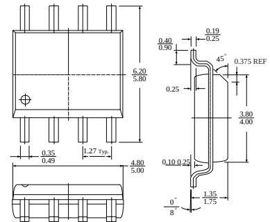
SOP-8
