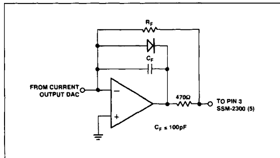
FIGURE 1: DAC Interface Circuit (SSM-2300 Single Supply, Op Amp Driver Split Supply)
