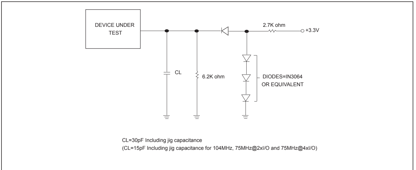
Figure 5. OUTPUT LOADING
