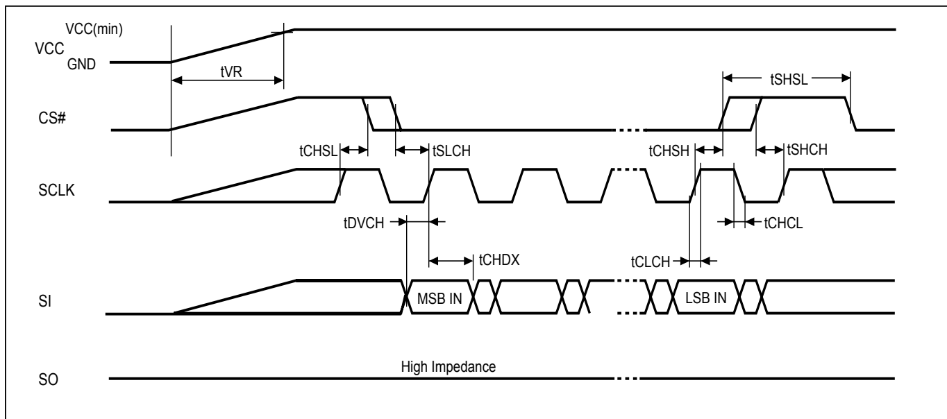
Figure 27. AC Timing at Device Power-Up
