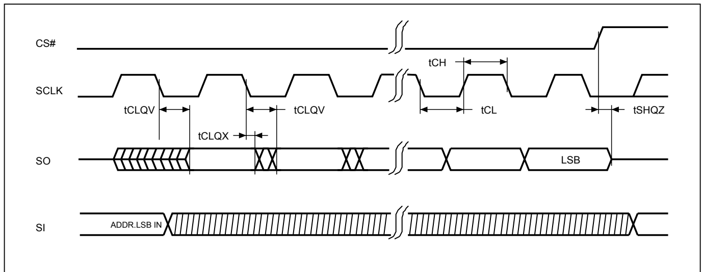
Figure 8. Output Timing
