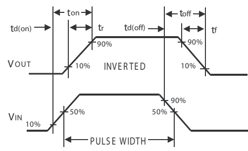
Figure 14. Switching Waveforms
