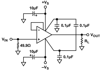
Figure 46. G = 1 Configuration
