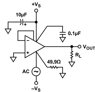
Figure 50. Negative Power Supply Rejection
