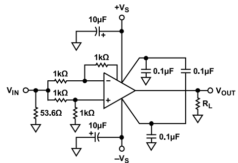
Figure 51. Common-Mode Rejection
