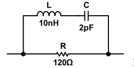
Figure 61. RLC Circuit
