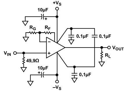
Figure 49. Noninverting Gain Configuration
