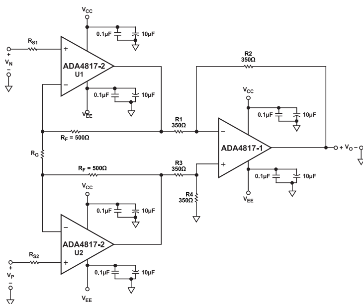
Figure 66. High Speed Instrumentation Amplifier
