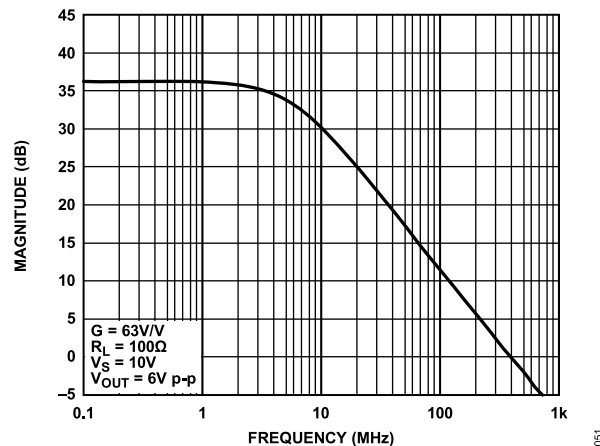
Figure 65. Photodiode Preamp Frequency Response
