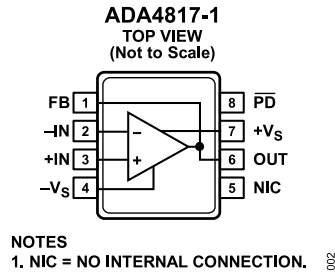
Figure 2. 8-Lead SOIC (RD-8-4)
