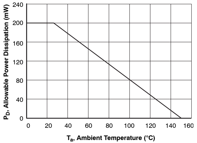
Figure 12. P_D - T_a
