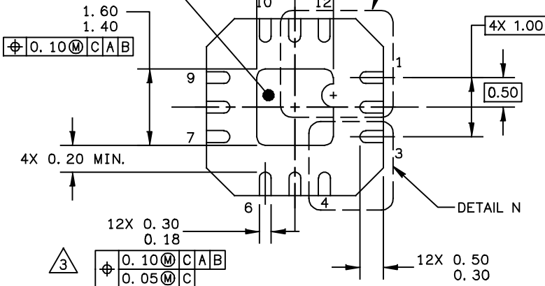
VIEW M-M
