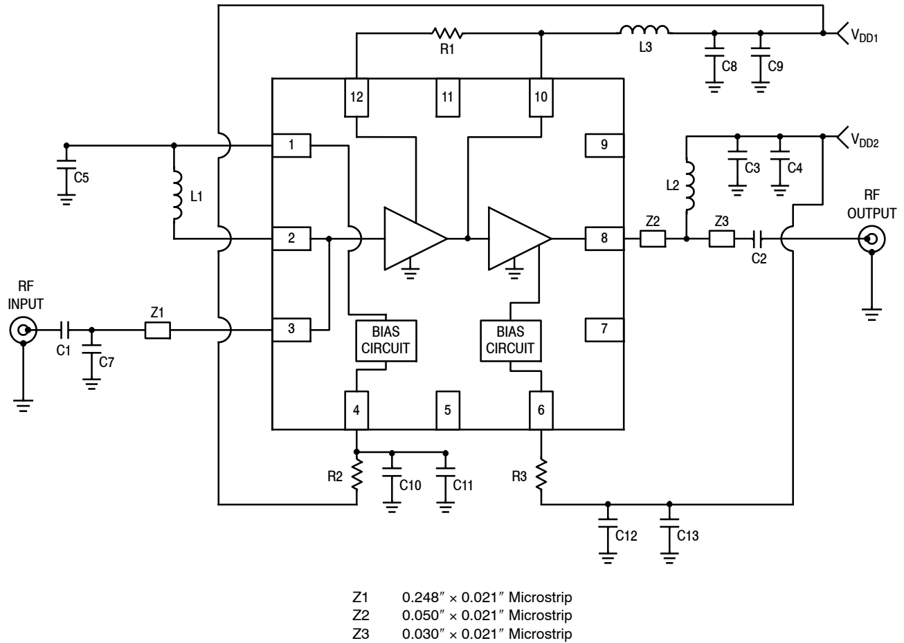
Figure A-1. MML20242HT1 Test Circuit Schematic
