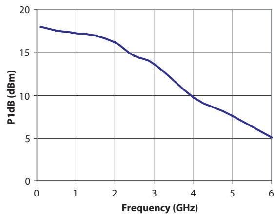
Figure 6. P1dB vs Frequency at I_d = 60\text{ mA} .
