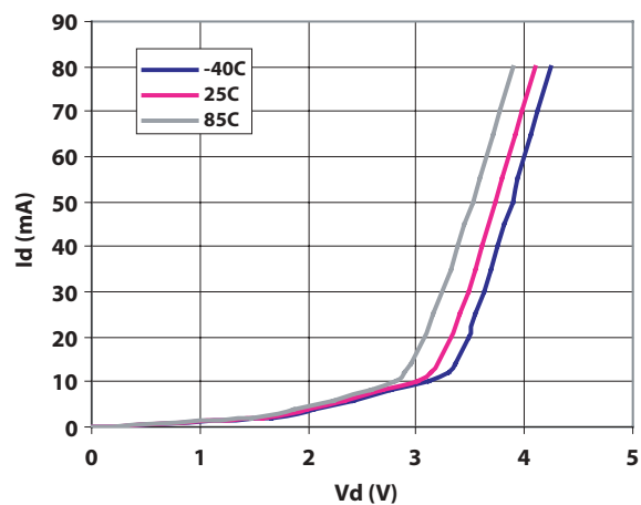
Figure 9. I_d vs. V_d and Temperature.
