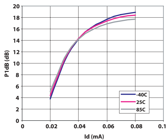
Figure 11. P1dB vs. I_d and Temperature at 900 MHz.
