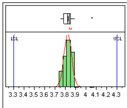
Figure 1. Vd Distribution@60mA.
