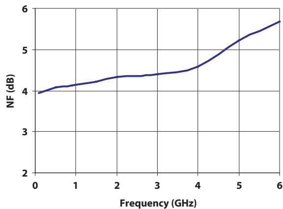
Figure 8. NF vs Frequency at I_d = 60 mA.
