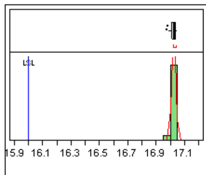
Figure 3. P1dB Distribution@60mA
