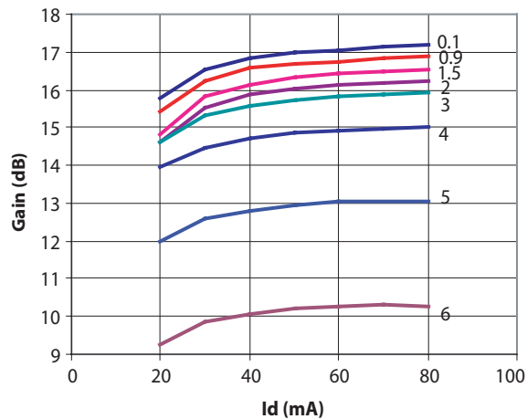
Figure 14. Gain vs Id and Frequency (GHz).
