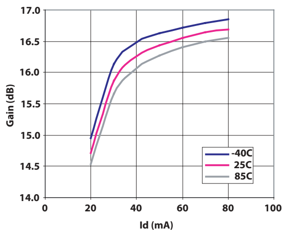
Figure 10. Gain vs. I_d and Temperature at 900 MHz.
