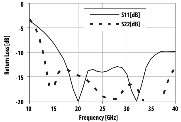
Figure 2. Return Loss vs Frequency
