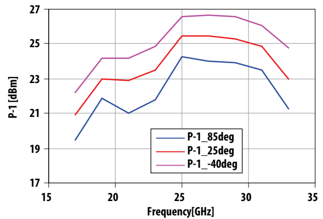
Figure 16. P_{-1\text{dB}} vs frequency and Temperature
