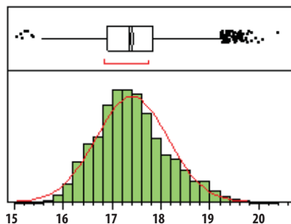
Gain at 33GHz
