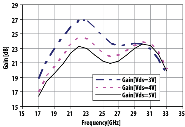
Figure 9. Small signal gain vs Frequency and Vds, ( I_{dQ}=230\text{mA} )
