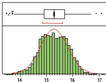
Gain at 17GHz
