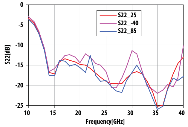
Figure 14. |S_{22}| vs Frequency and Temperature
