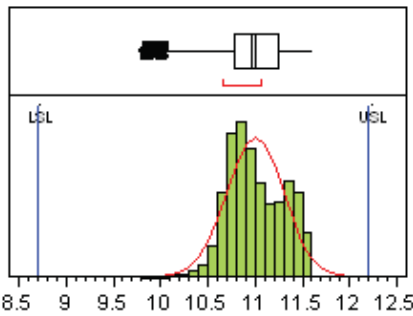
Figure 3. Gain @ 12 GHz, LSL=8.7, Nominal=11.0, USL=12.2, CPK=1.3
