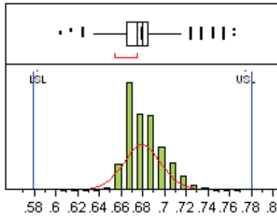
Figure 2. Gate Voltage @ V_{ds} = 2V & I_{ds} = 20mA , LSL=0.58, Nominal=0.68, USL=0.78, CPK=1.9
