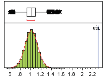
Figure 4. NF @ 12 GHz, Nominal=1.0, USL=2.3, CPK=3.5
