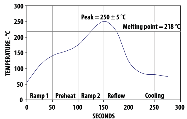
Figure 19. Suggested Lead-Free Reflow Profile for SnAgCu Solder Paste
