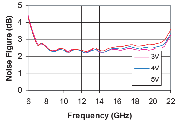
Figure 10b. Noise Figure Over V_{dd}
