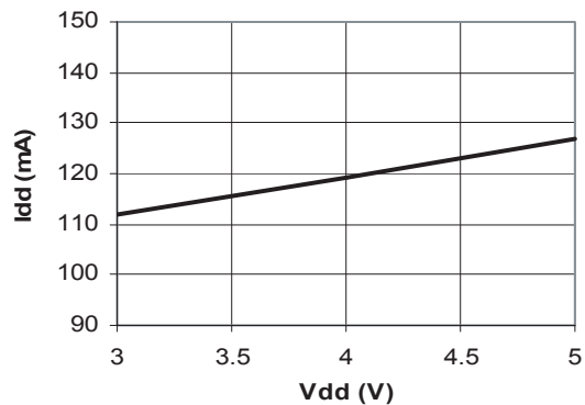
Figure 8a. I_{dd} over V_{dd}
