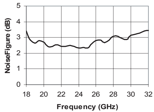
Figure 2. Noise Figure
