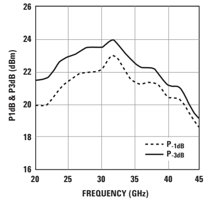
Figure 9. Output Power at P_{1dB} and P_{3dB} , V_{DD}=4.5 V, I_{DD}=300 mA.
