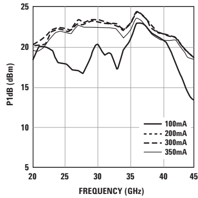
Figure 8. Output Power ( P_{1dB} ) and Drain Current, V_{DD}=4.5 V.
