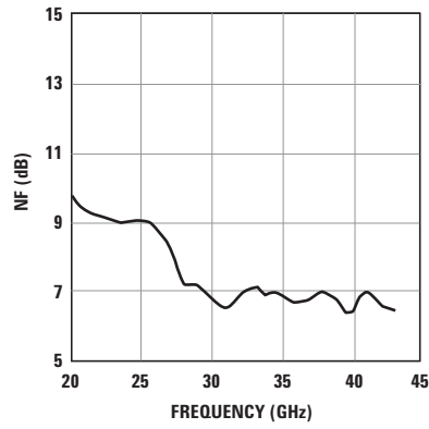
Figure 10. Noise Figure, V_{DD}=4.5 V, I_{DD}=300 mA.
