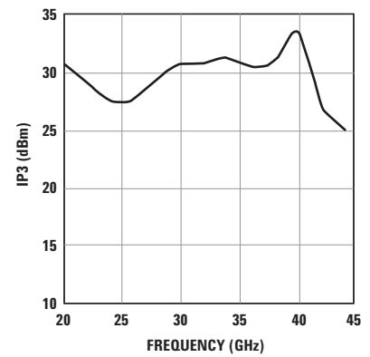
Figure 12. Output 3 rd Order Intercept Point, V_{DD}=4.5 V, I_{DD}=300 mA.
