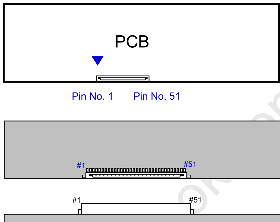
Fig. Connector diagram
