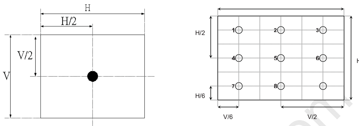
FIG. 2 Luminance
