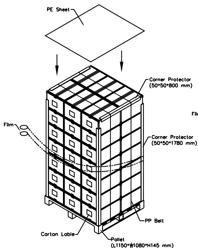
Figure. 7-3 Packing method
