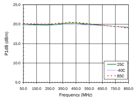
P_{1dB} versus Frequency
