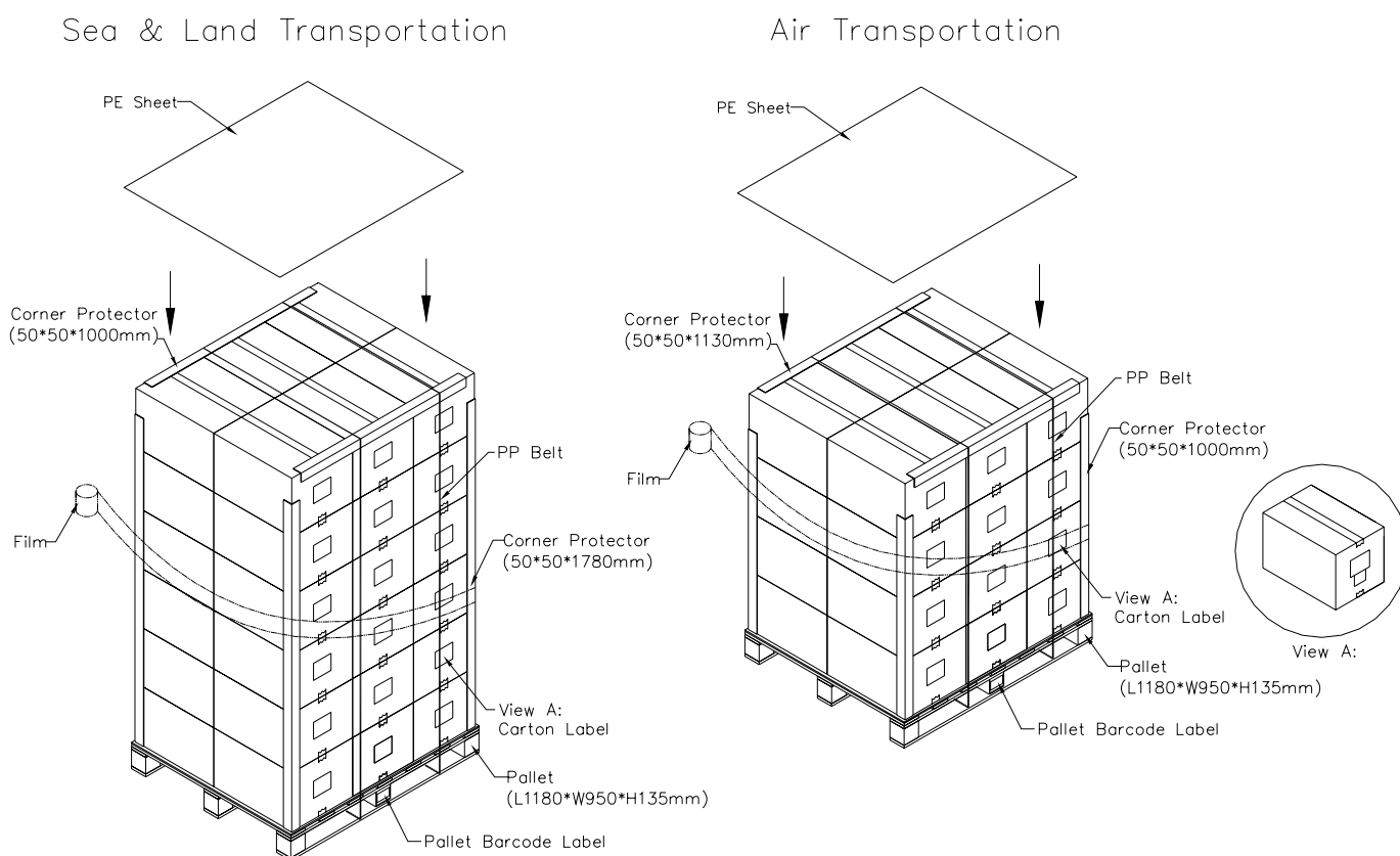
Figure. 7-3 Packing method
