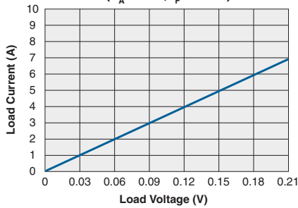
CPC1718 Typical Load Current vs. Load Voltage ( T_A=25^{\circ}C , I_F=10mA )
