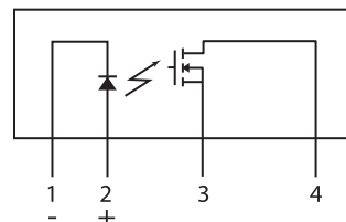
CPC1726 Pinout
