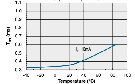
Typical Turn-On Time vs. Temperature ( V_L=10\text{V} , R_L=1\text{k}\Omega )
