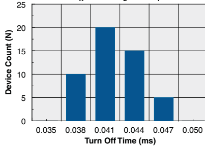
Typical Turn-Off Time Distribution (N=50, T_A=25^\circ\text{C} , V_L=10\text{V} , I_F=10\text{mA} )
