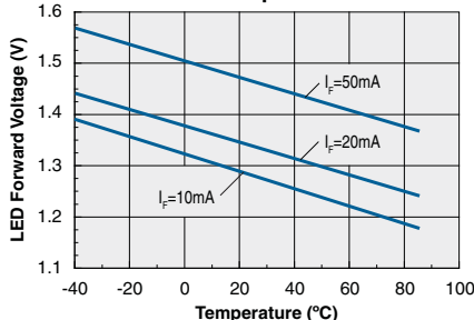
Typical LED Forward Voltage vs. Temperature
