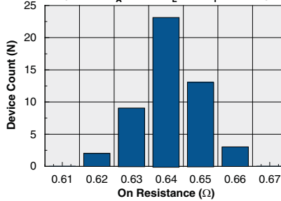
Typical On-Resistance Distribution (N=50, T_A=25^\circ\text{C} , I_L=1\text{A} , I_F=10\text{mA} )
