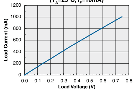
Typical Load Current vs. Load Voltage ( T_A=25^{\circ}C , I_F=10mA )
