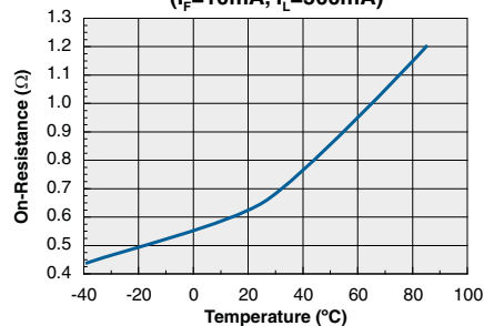
Typical On-Resistance vs. Temperature ( I_F=10mA , I_L=500mA )
