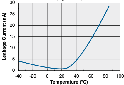
Typical Leakage Current vs. Temperature Measured Across Pins 3 & 4 ( V_L=250\text{V} )
