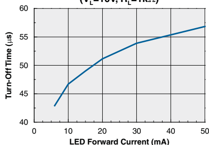
Typical Turn-Off Time vs. LED Forward Current ( V_L=10V , R_L=1k\Omega )
