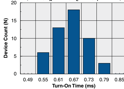
Typical Turn-On Time Distribution (N=50, T_A=25^\circ\text{C} , V_L=10\text{V} , I_F=10\text{mA} )
