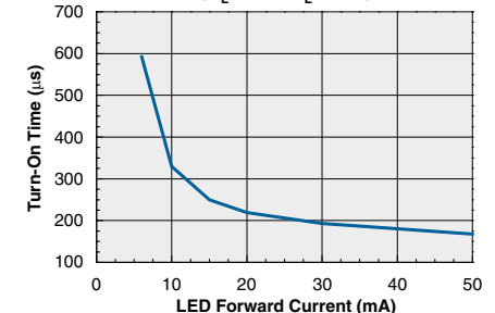
Typical Turn-On Time vs. LED Forward Current ( V_L=10\text{V} , R_L=1\text{k}\Omega )
