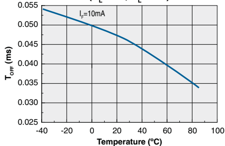
Typical Turn-Off Time vs. Temperature ( V_L=10\text{V} , R_L=1\text{k}\Omega )
