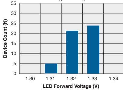
Typical LED Forward Voltage Drop ( N=50 , T_A=25^\circ\text{C} , I_F=10\text{mA} )
