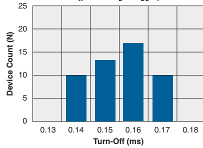
Typical Turn-Off Time ( N=50 , T_A=25^\circ\text{C} , I_L=1A_{DC} , I_F=20\text{mA} )
