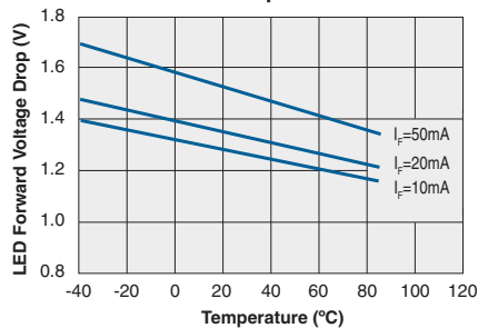
Typical Forward Voltage Drop vs. Temperature
