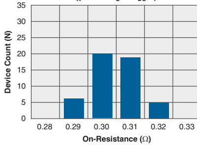
Typical On-Resistance Distribution ( N=50 , T_A=25^\circ\text{C} , I_L=1A_{DC} , I_F=10\text{mA} )
