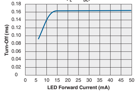
Typical Turn-Off vs. LED Forward Current ( I_L=1A_{DC} )
