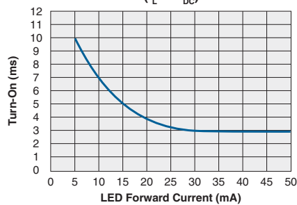
Typical Turn-On vs. LED Forward Current ( I_L=1A_{DC} )
