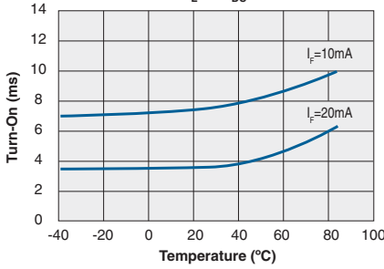
Typical Turn-On vs. Temperature ( I_L=1A_{DC} )
