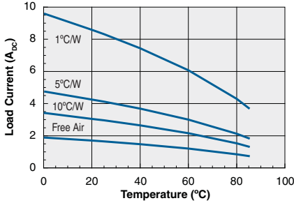
Maximum Load Current vs. Temperature with Heat Sink
