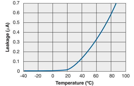
Typical Leakage vs. Temperature at Maximum Rated Voltage (Measured Across Pins 1 & 2)
