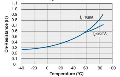
Typical On-Resistance vs. Temperature ( I_L = \text{Max Rated} )
