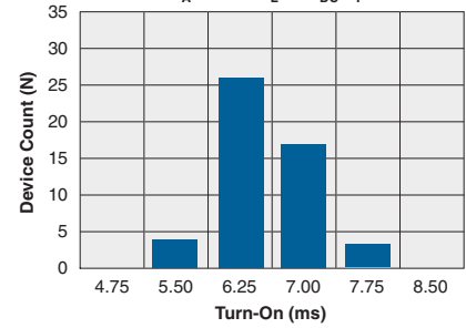
Typical Turn-On Time ( N=50 , T_A=25^\circ\text{C} , I_L=1A_{DC} , I_F=20\text{mA} )
