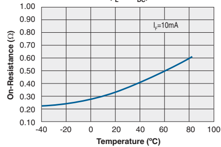
Typical On-Resistance vs. Temperature ( I_L = 1A_{DC} )
