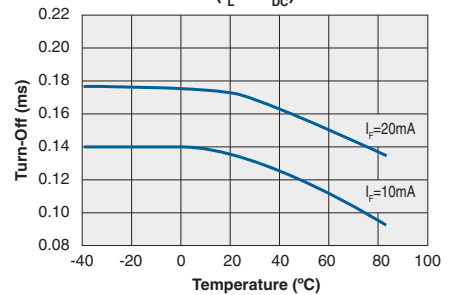
Typical Turn-Off vs. Temperature ( I_L=1A_{DC} )
