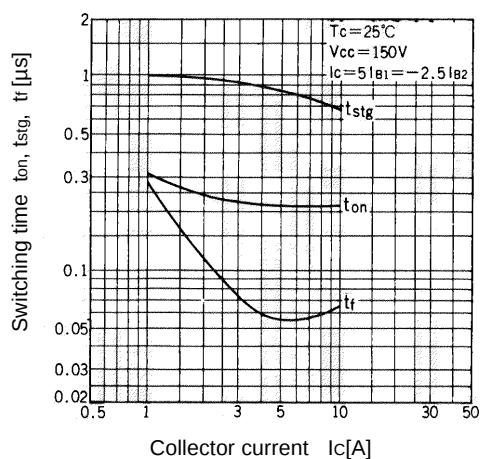
Switching Time
