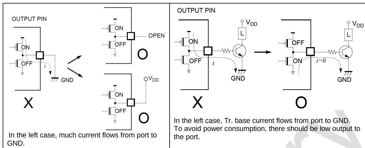
Figure 27-7 Application Example of Unused Output Port
