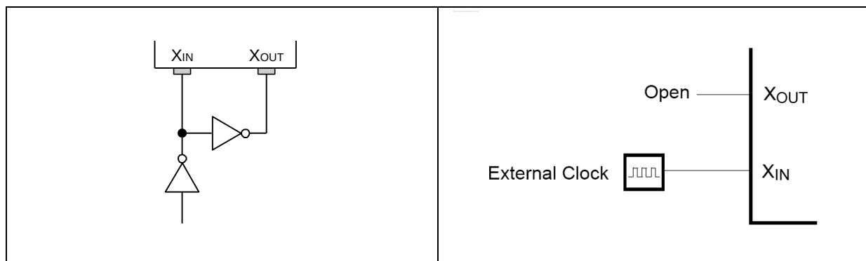
Figure 14-6 External Clock
