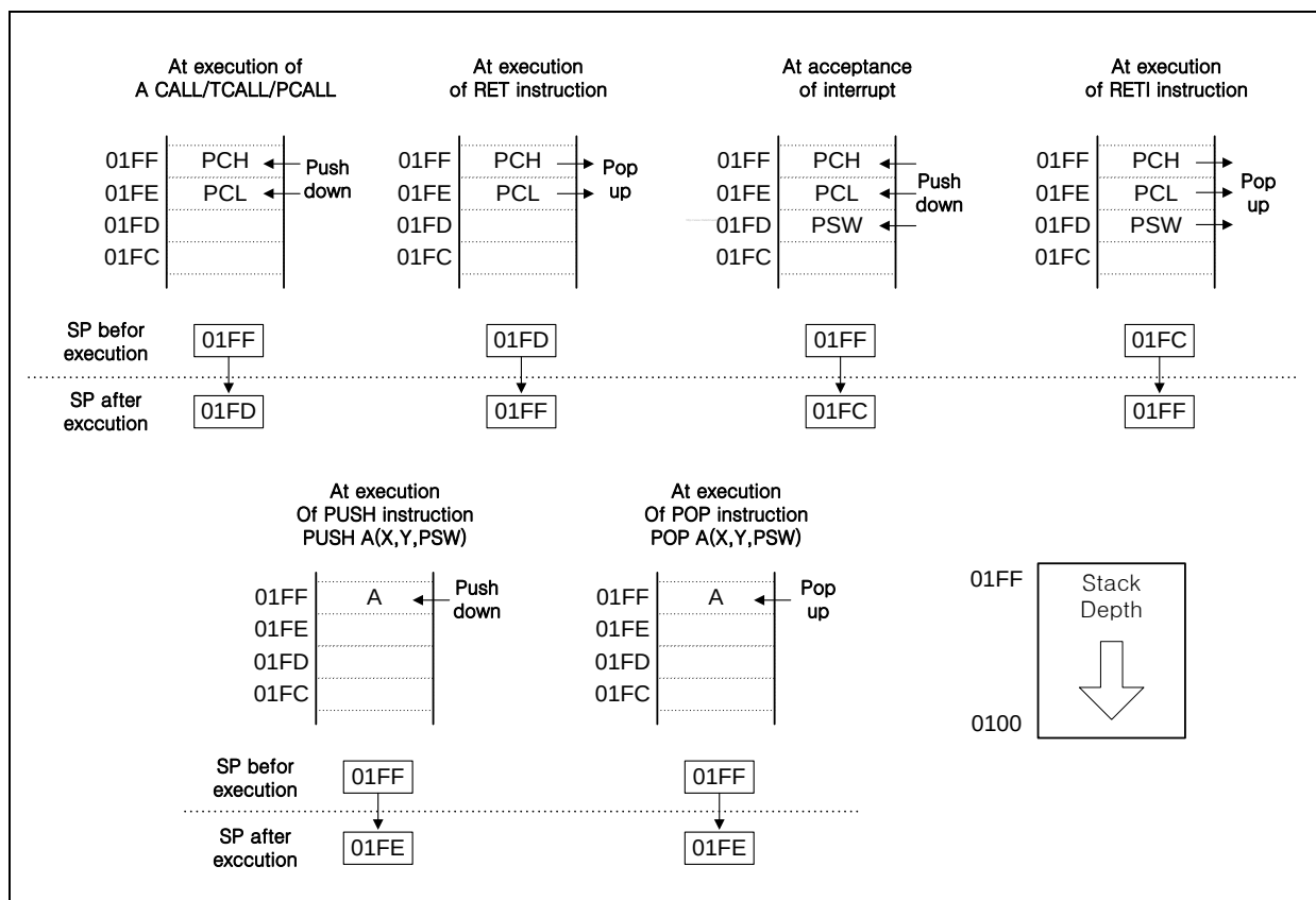
Figure 9-4 Stack Operation
