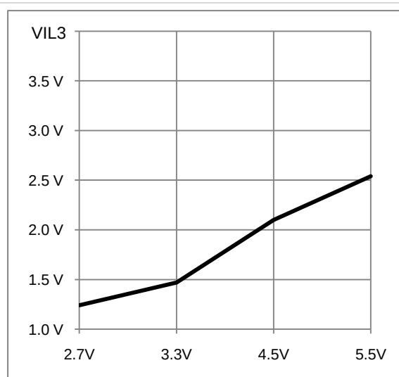
Figure 7-26 V IL3 - V DD
