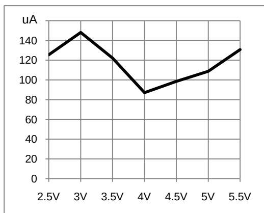
Figure 7-14 I DD2 – V DD in Sub Active Mode
