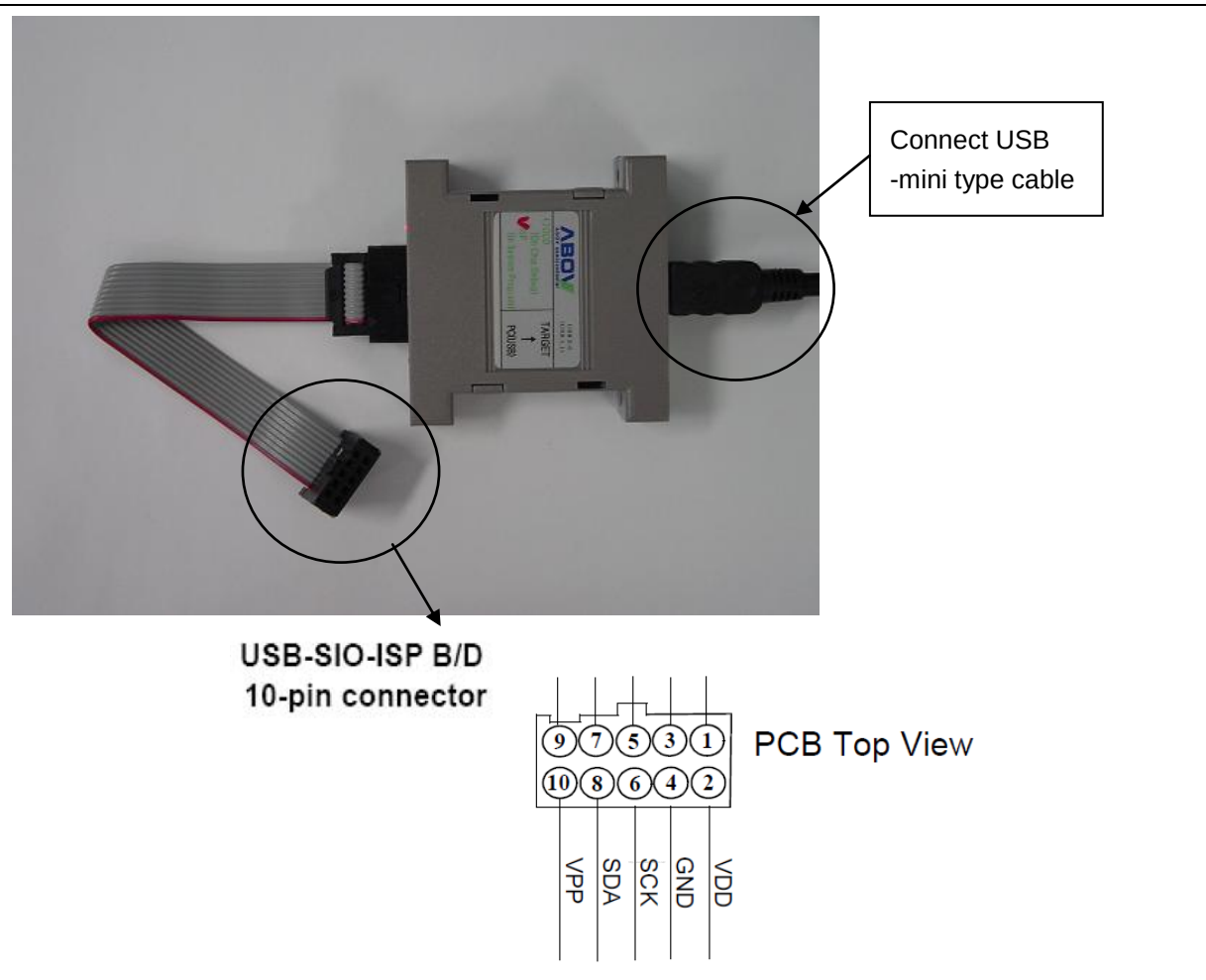
Figure 29-3 USB-SIO-ISP Board
