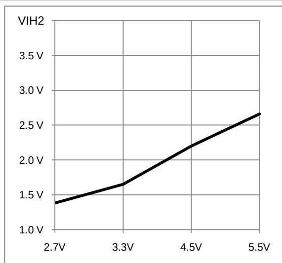
Figure 7-23 V IH2 - V DD
