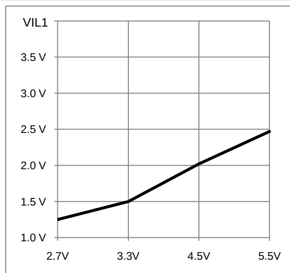
Figure 7-22 V IL1 - V DD
