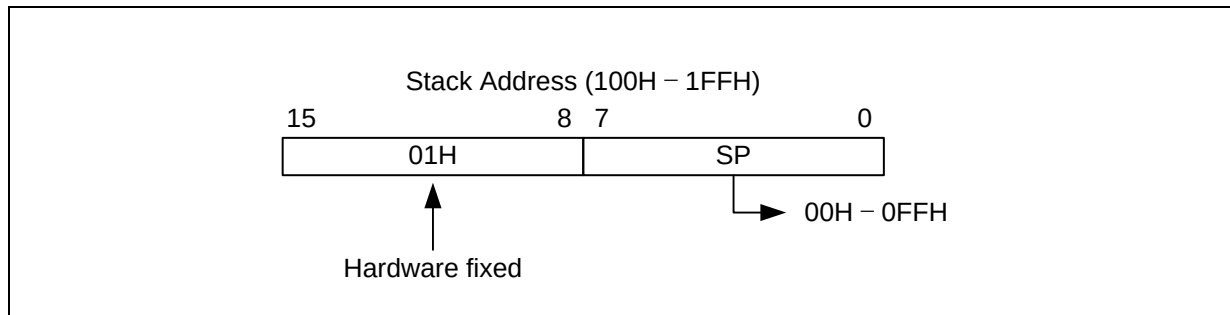
Figure 9-3 Stack Pointer
