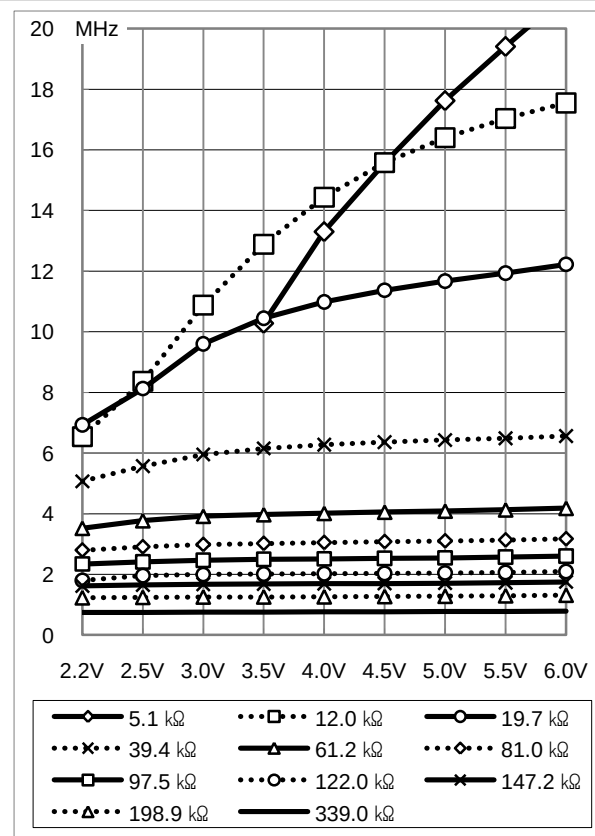
Figure 7-29 Ext. R/C OSC Freq. - V_{DD} at 85^{\circ}\text{C}
