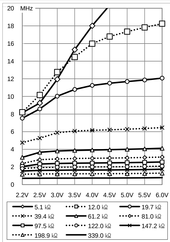
Figure 7-30 Ext. R/C OSC Freq. - V_{DD} at -40^{\circ}\text{C}
