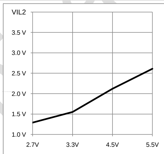
Figure 7-24 V IL2 - V DD
