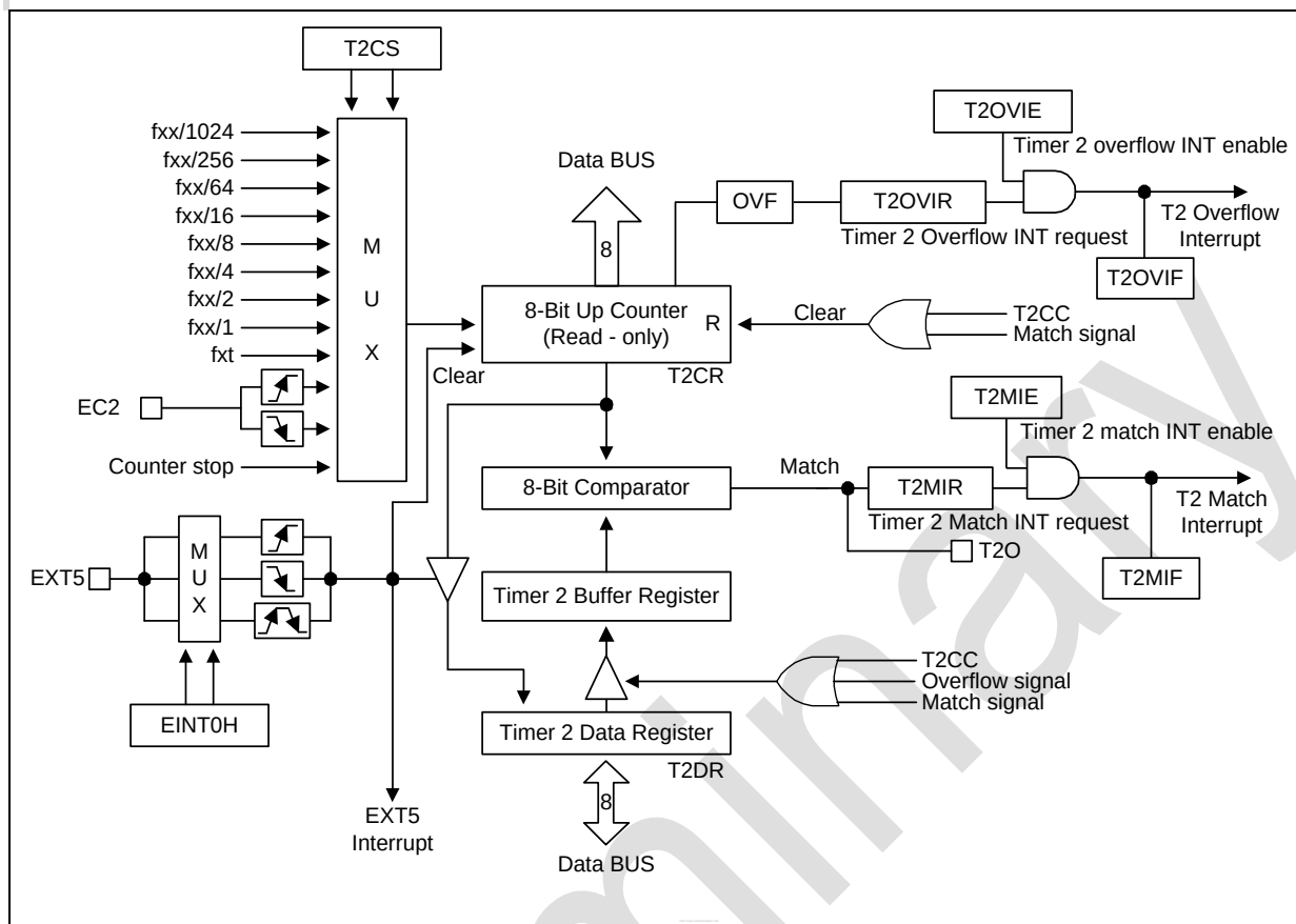
Figure 19-1 8-bit Timer 2 Block Diagram
