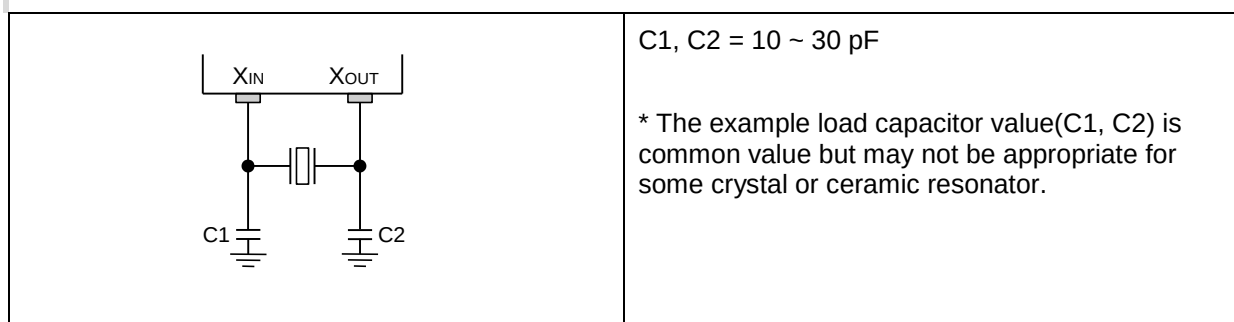
Figure 14-5 Crystal/Ceramic Oscillator
