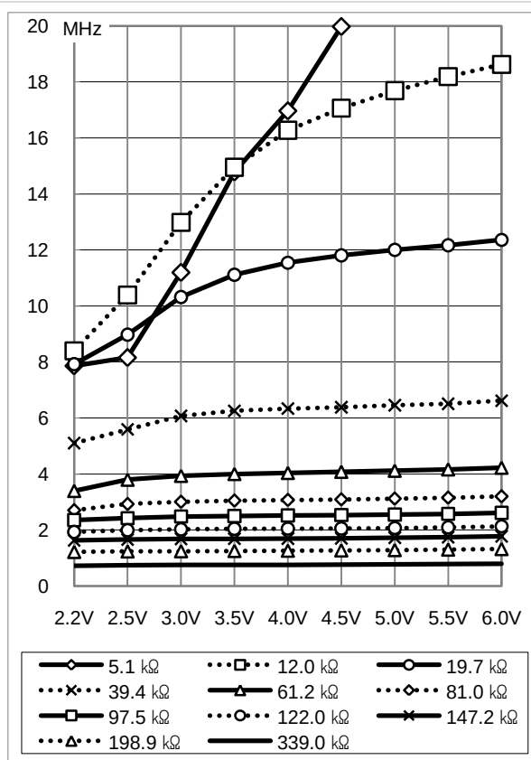
Figure 7-28 Ext. R/C OSC Freq. - V_{DD} at 25^{\circ}\text{C}
