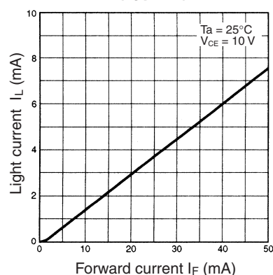
Light Current vs. Forward Current Characteristics (Typical)
