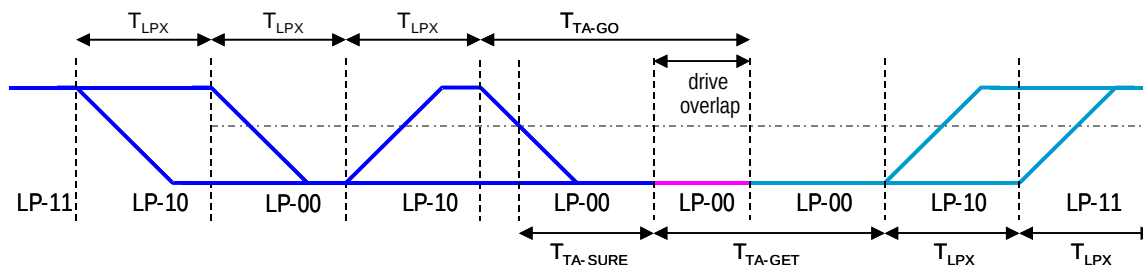
Figure 9-5: Turnaround Procedure
