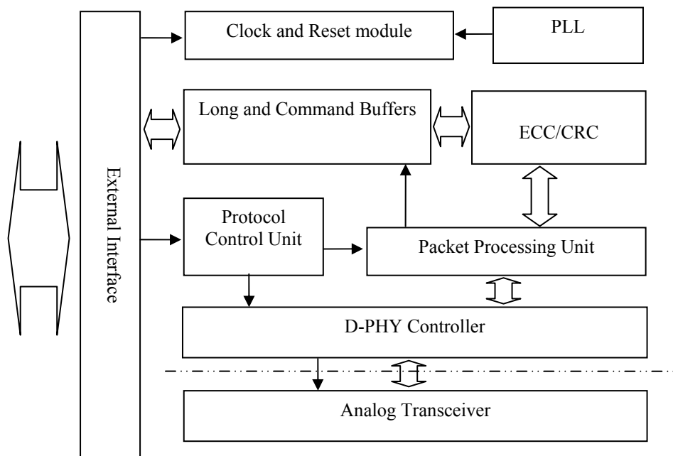
Figure 4-3: Block Diagram
