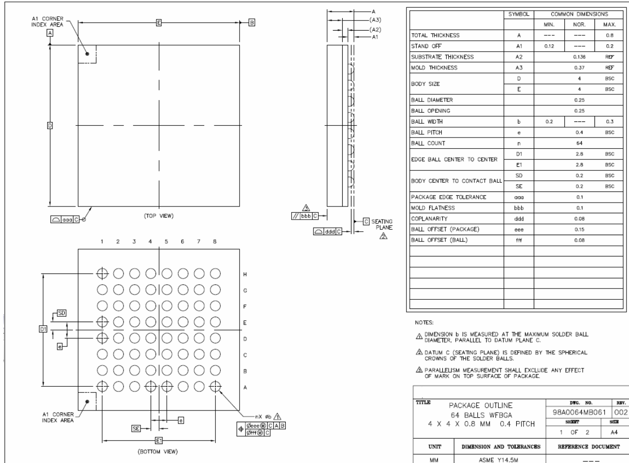
Figure 18-1- Package Information
