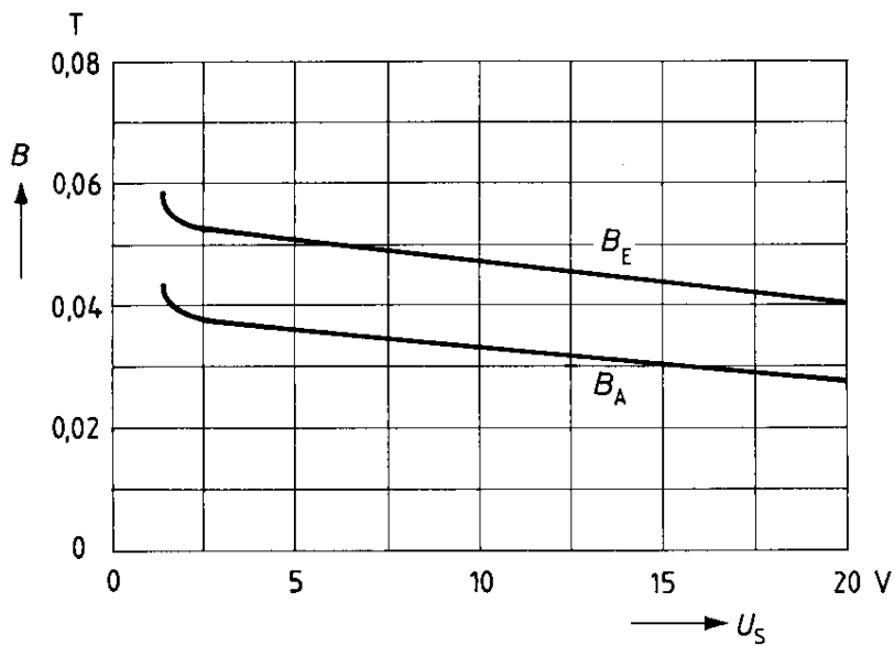
B_E, B_A = f(U_S) , typ.
