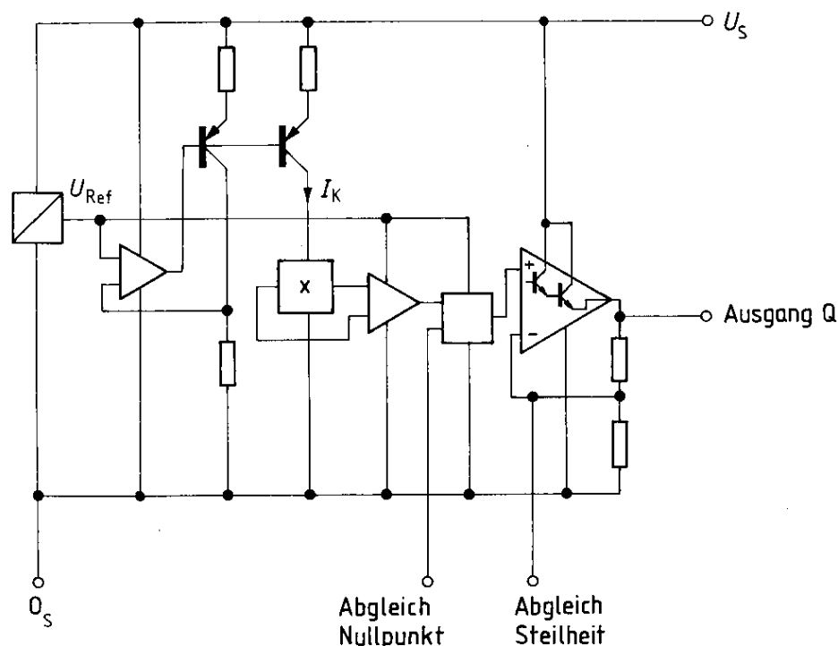
Lineare Hall-IS
