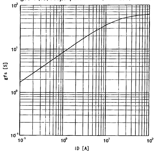
Typical Transconductance
