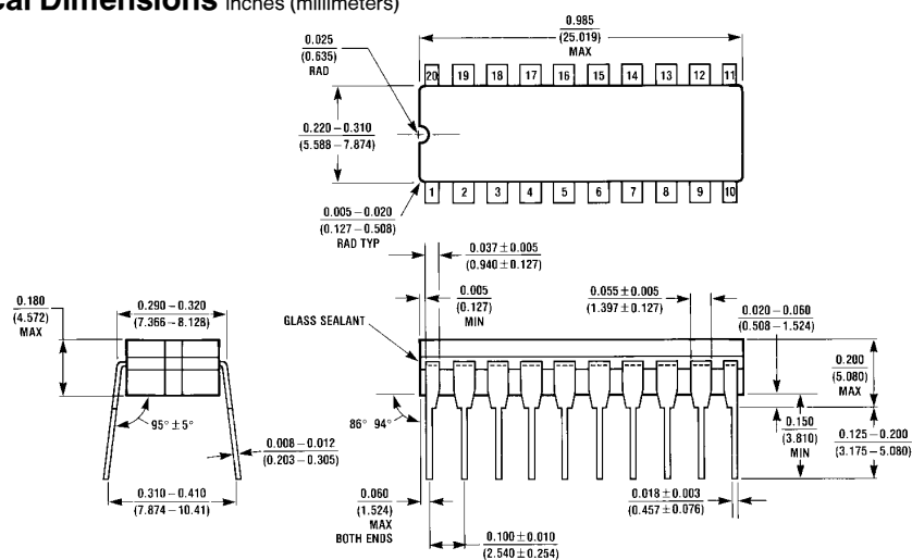
Order Number MM54HCT688J or MM74HCT688J NS Package J20A
